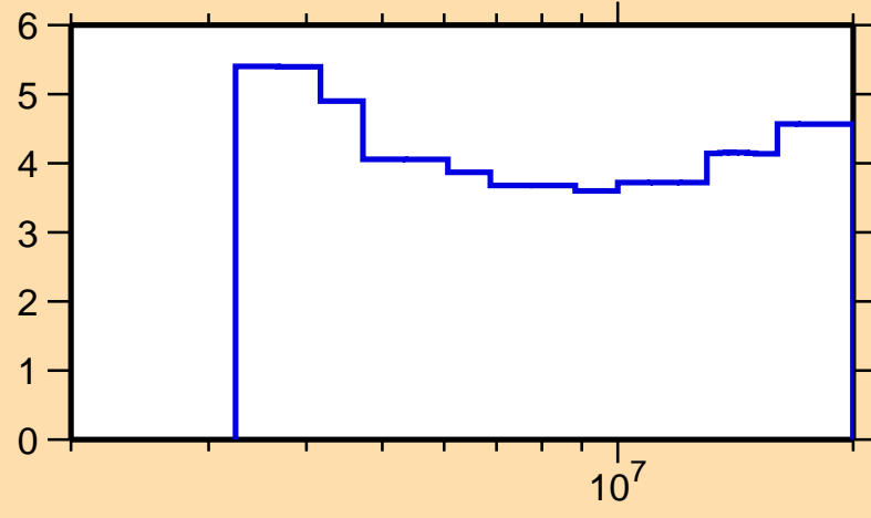
\Delta\sigma/\sigma vs. E for ^{94}\text{Zr}(n, n_{\text{nonel}})
