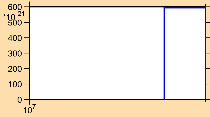
\sigma vs. E for ^{94}\text{Zr}(n,3n\alpha)
