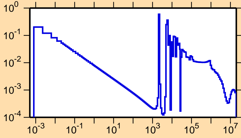
\sigma vs. E for ^{94}\text{Zr}(n,\gamma)
