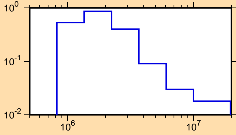
\sigma vs. E for ^{94}\text{Zr}(n,n_1)
