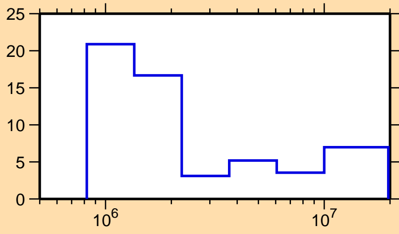
\Delta\sigma/\sigma vs. E for ^{94}\text{Zr}(n,\text{tot.})
