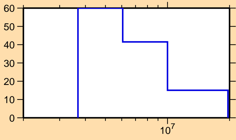
\Delta\sigma/\sigma vs. E for ^{94}\text{Zr}(n,p)
