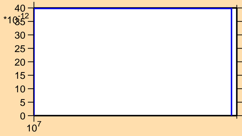
\sigma vs. E for ^{94}\text{Zr}(n,nt)
