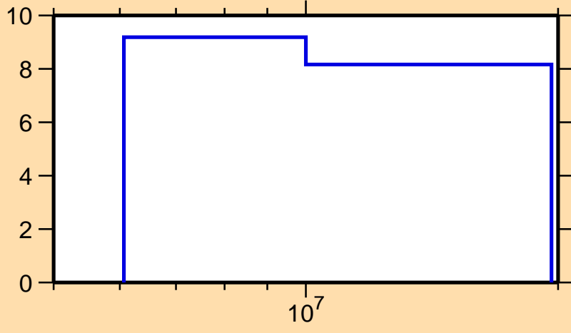
\Delta\sigma/\sigma vs. E for ^{94}\text{Zr}(n,2n)
