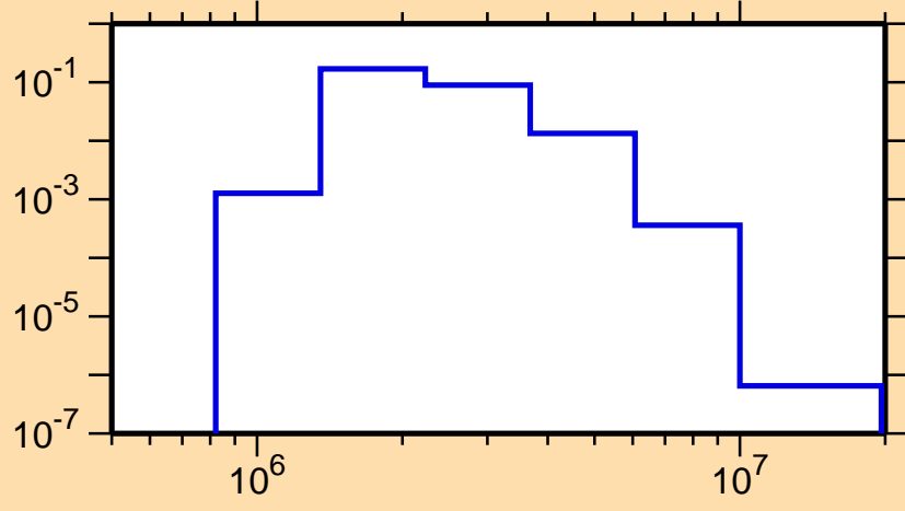
\sigma vs. E for ^{94}\text{Zr}(n,n_2)
