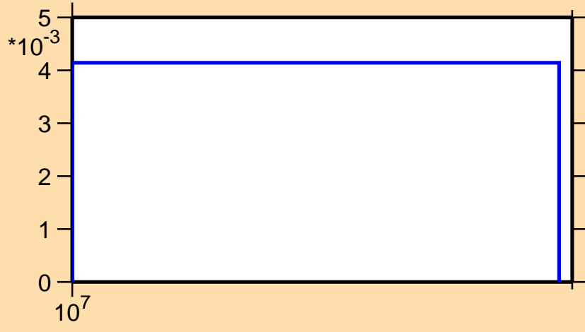
\sigma vs. E for ^{94}\text{Zr}(n,3n)
