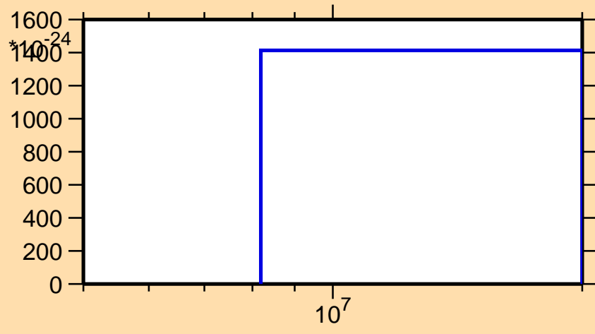
\sigma vs. E for ^{94}\text{Zr} (mt 34)
