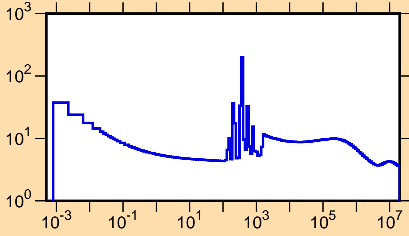
\sigma vs. E for ^{95}\text{Zr}(n,\text{tot.})
