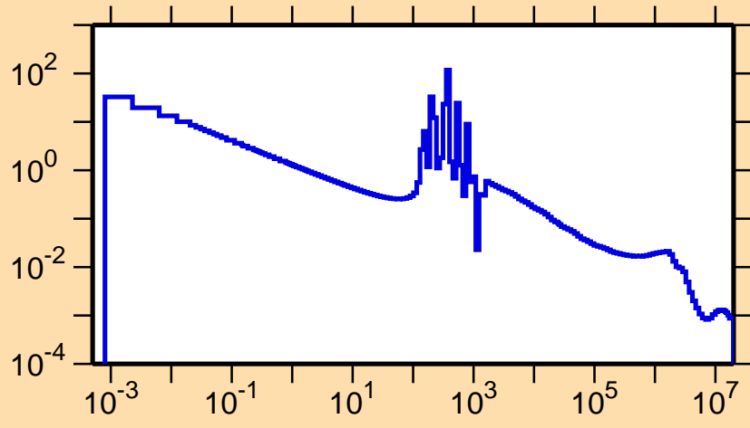
\sigma vs. E for ^{95}\text{Zr}(n,\gamma)
