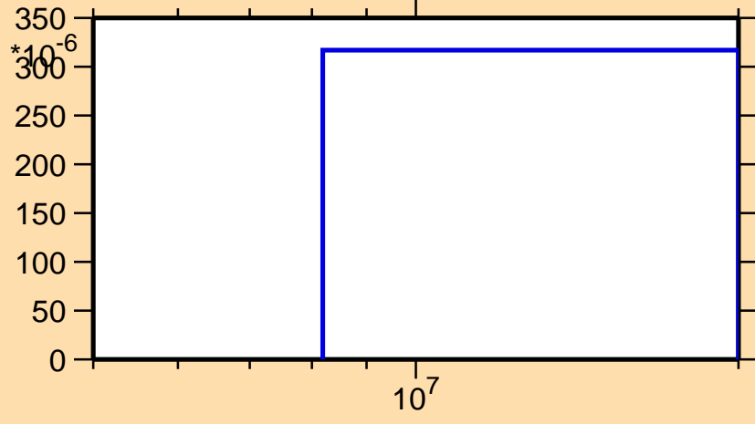
\sigma vs. E for ^{95}\text{Zr}(n,d)
