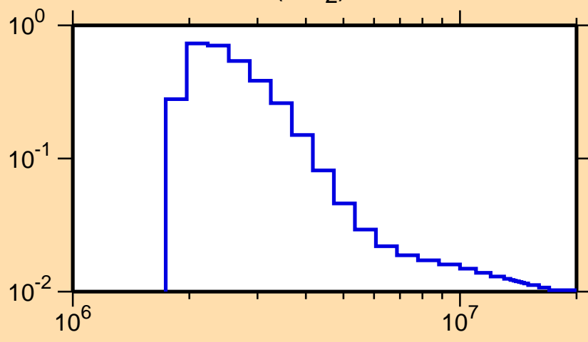
\sigma vs. E for ^{96}\text{Zr}(n,n_2)
