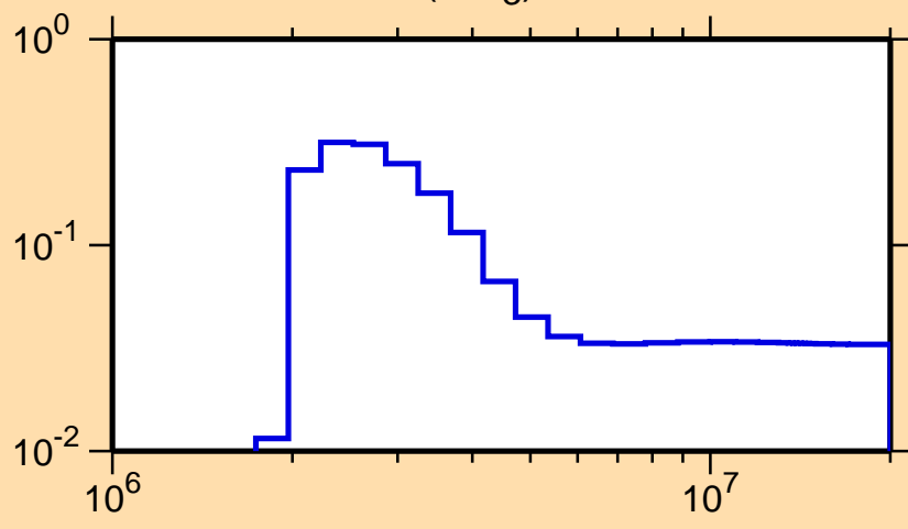
\sigma vs. E for ^{96}\text{Zr}(n,n_3)
