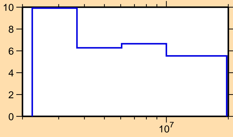
\Delta\sigma/\sigma vs. E for ^{96}\text{Zr}(n,n\text{onel.})
