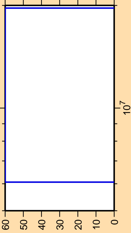
\Delta\sigma/\sigma vs. E for ^{96}\text{Zr}(n,\gamma)
