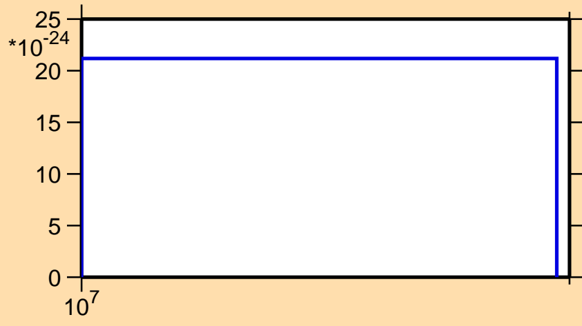
\sigma vs. E for ^{97}\text{Zr}(n,3n\alpha)
