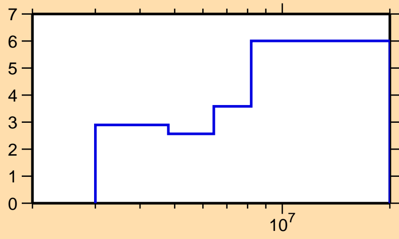
\Delta\sigma/\sigma vs. E for ^{97}\text{Zr}(n,\text{tot.})
