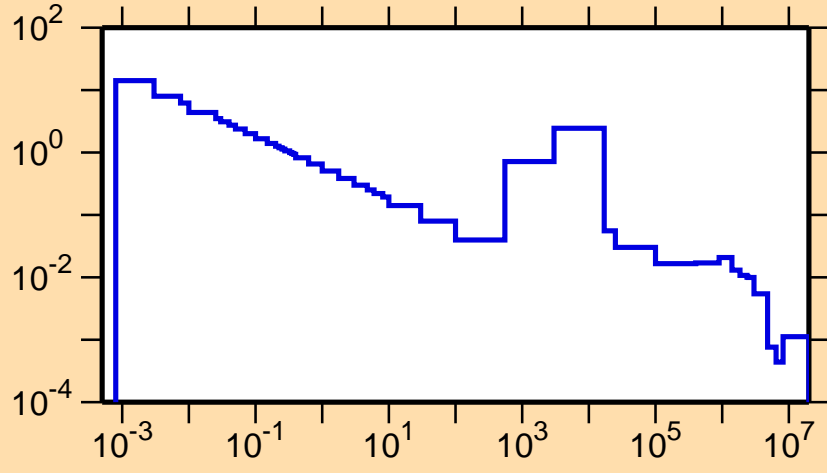
\sigma vs. E for ^{97}\text{Zr}(n,\gamma)
