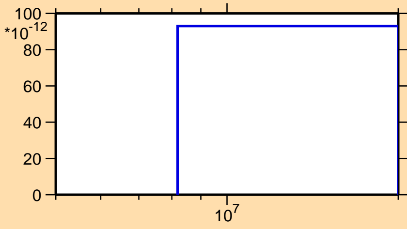
\sigma vs. E for ^{97}\text{Zr}(n,nt)
