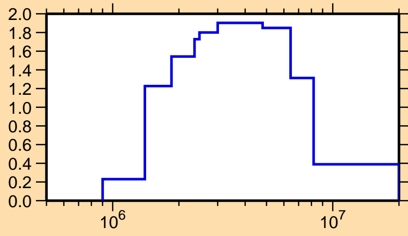
\sigma vs. E for ^{97}\text{Zr}(n,\text{inel.})
