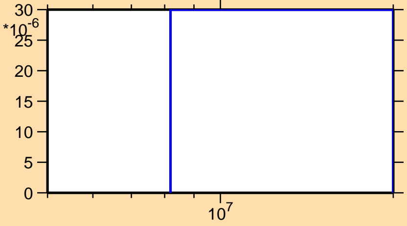
\sigma vs. E for ^{97}\text{Zr}(n,n\alpha)
