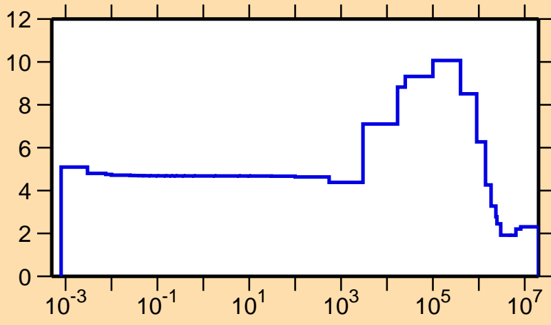
\sigma vs. E for ^{97}\text{Zr}(n,\text{el.})
