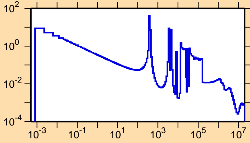
\sigma vs. E for ^{98}\text{Zr}(n,\gamma)
