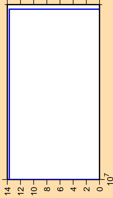
\Delta\sigma/\sigma vs. E for ^{98}\text{Zr}(n,nd)
