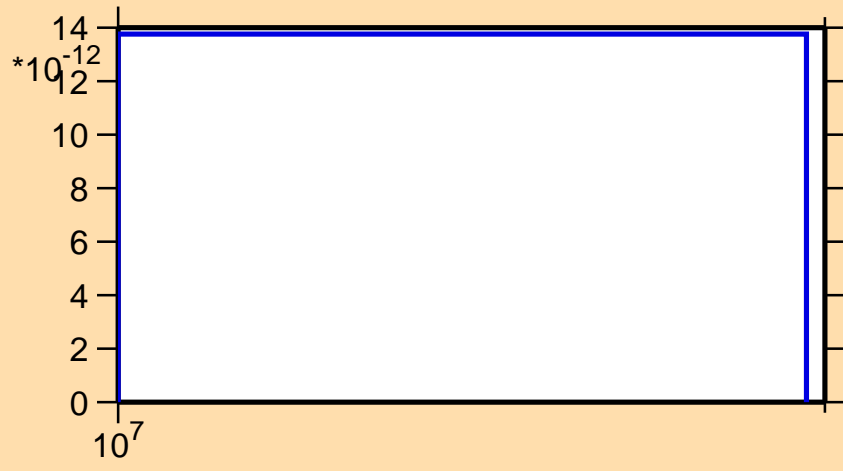
\sigma vs. E for ^{98}\text{Zr}(n,nd)
