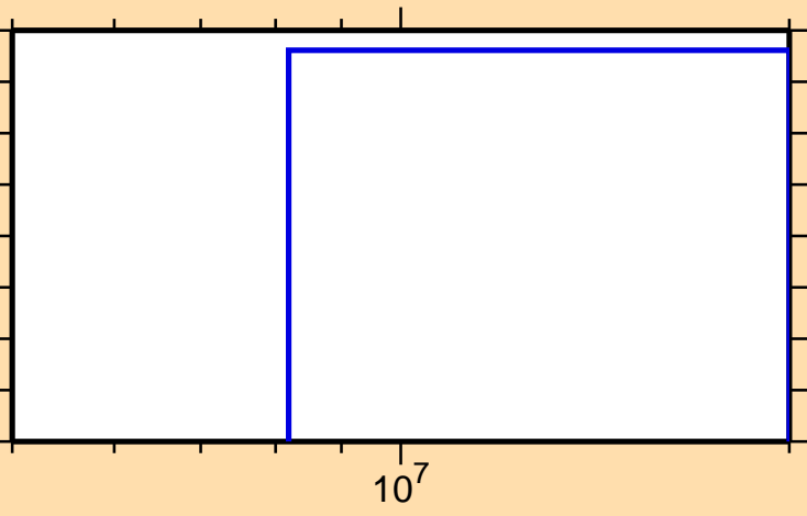
\sigma vs. E for ^{98}\text{Zr}(n,n\alpha)
