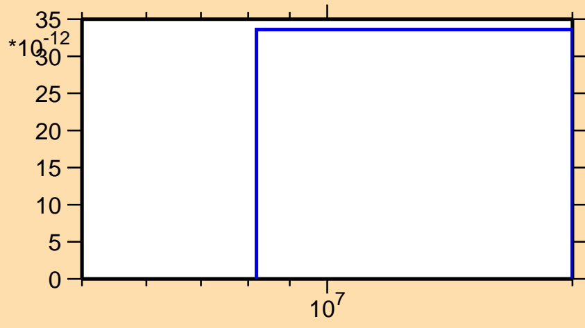
\sigma vs. E for ^{98}\text{Zr}(n,2n\alpha)
