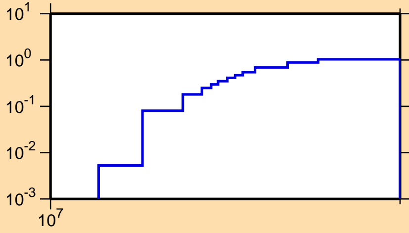
\sigma vs. E for ^{100}\text{Zr}(n,3n)
