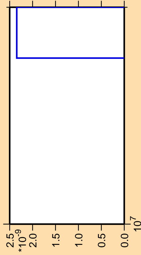
\Delta\sigma/\sigma vs. E for ^{100}\text{Zr}(n,2np)
