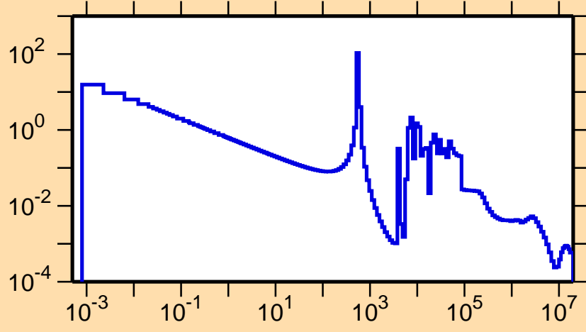
\sigma vs. E for ^{100}\text{Zr}(n,\gamma)
