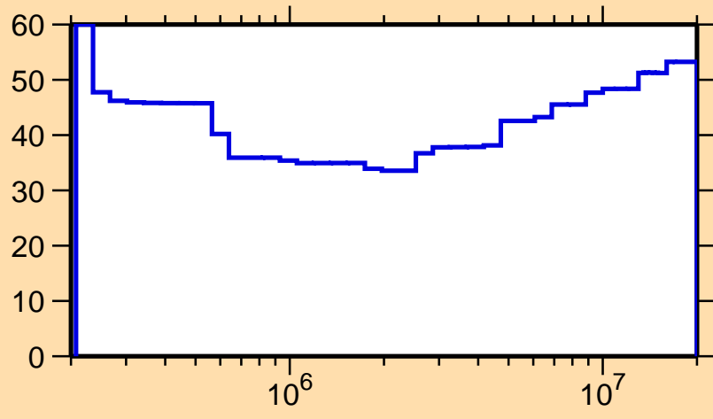
\Delta\sigma/\sigma vs. E for ^{100}\text{Zr}(n,n_1)
