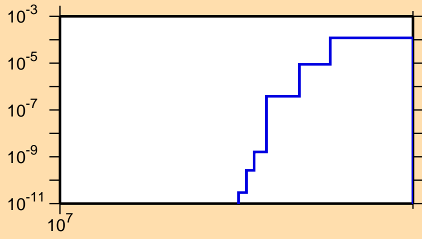
\sigma vs. E for ^{100}\text{Zr}(n,np)
