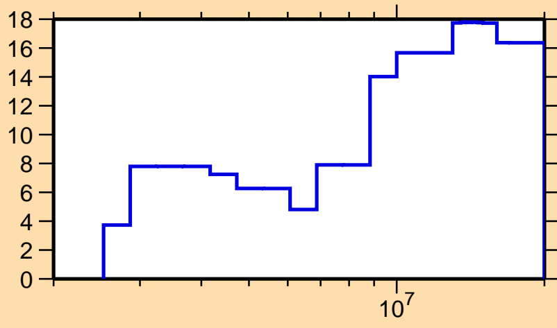
\Delta\sigma/\sigma vs. E for ^{100}\text{Zr}(n, el.)
