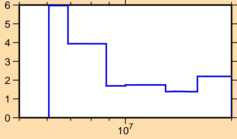
\Delta\sigma/\sigma vs. E for ^{100}\text{Zr}(n,\text{nonel.})
