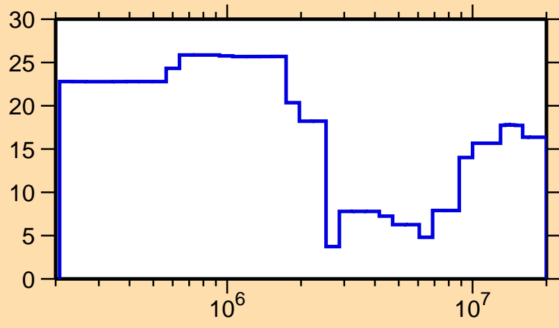
\Delta\sigma/\sigma vs. E for ^{100}\text{Zr}(n,\text{el.})
