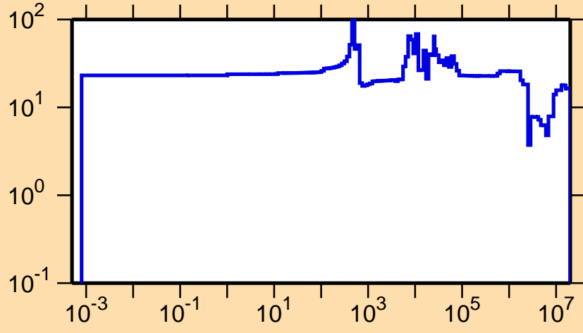
\Delta\sigma/\sigma vs. E for ^{100}\text{Zr}(n,\text{el.})
