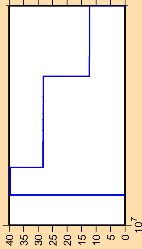
\Delta\sigma/\sigma vs. E for ^{100}\text{Zr}(n,3n)
