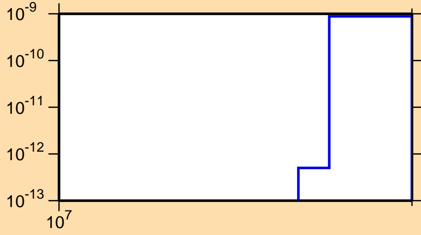
\sigma vs. E for ^{100}\text{Zr}(n,2n\alpha)
