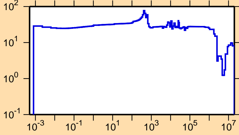
\Delta\sigma/\sigma vs. E for ^{100}\text{Zr}(n,\text{tot.})
