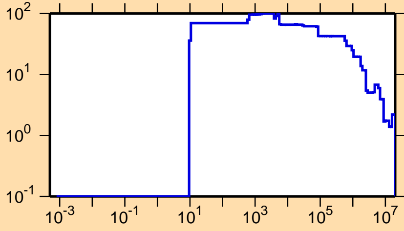
\Delta\sigma/\sigma vs. E for ^{100}\text{Zr}(n,\text{nonel.})
