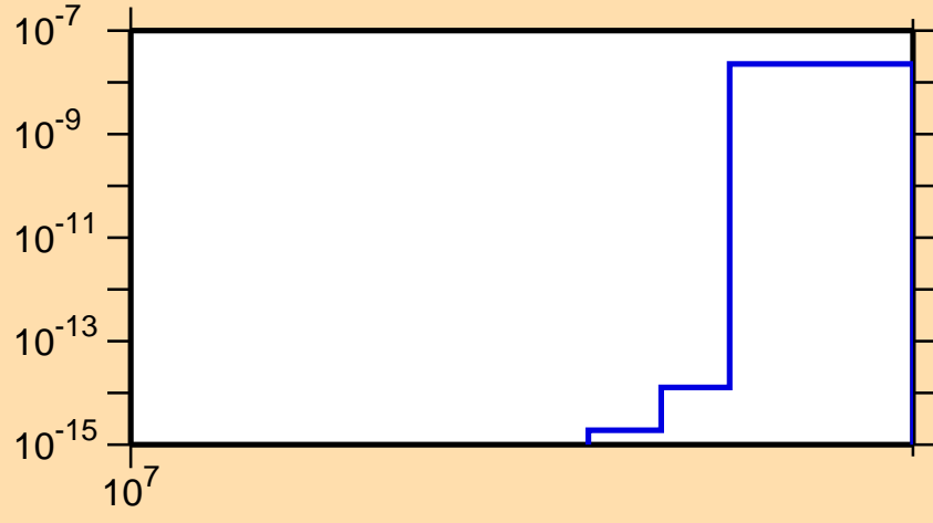
\sigma vs. E for ^{100}\text{Zr}(n,nt)
