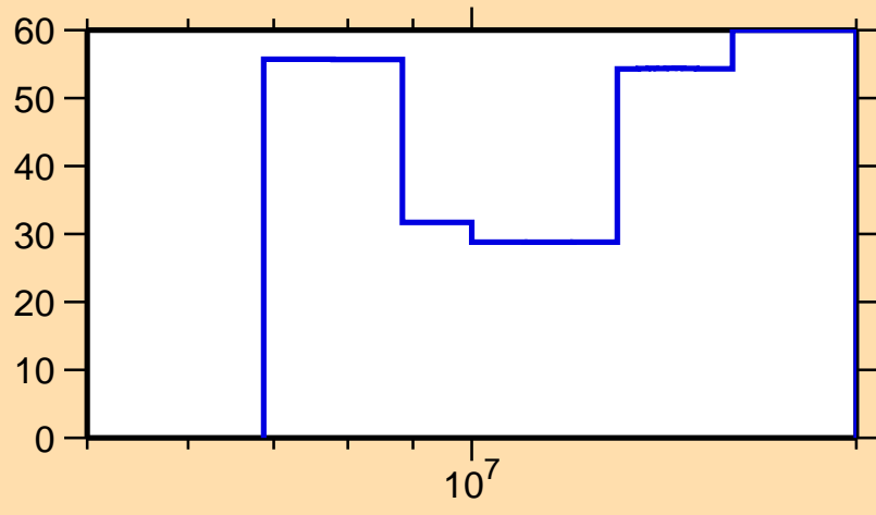
\Delta\sigma/\sigma vs. E for ^{100}\text{Zr}(n,2n)
