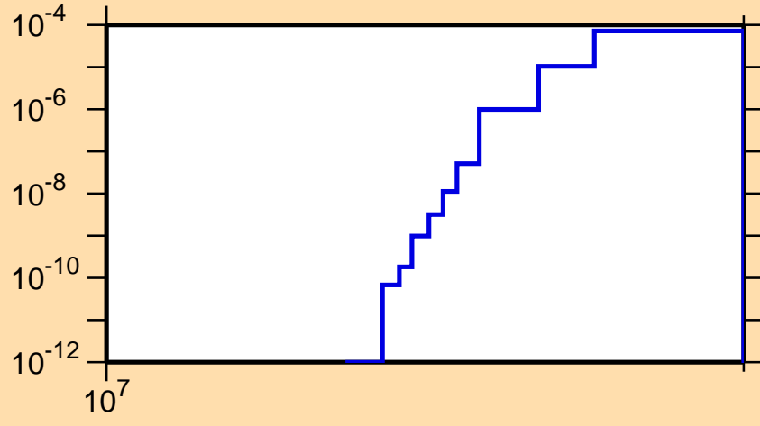
\sigma vs. E for ^{100}\text{Zr}(n,t)
