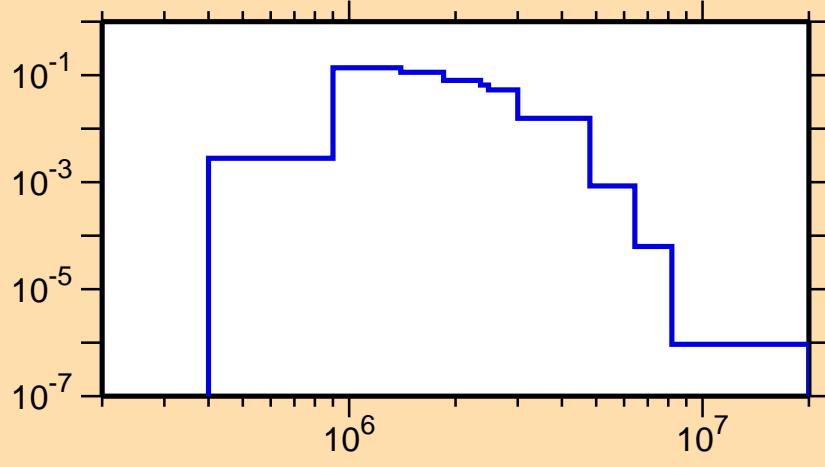
\sigma vs. E for ^{100}\text{Zr}(n,n_4)
