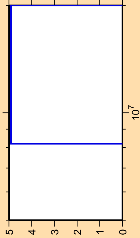
\Delta\sigma/\sigma vs. E for ^{100}\text{Zr}(n,2n\alpha)
