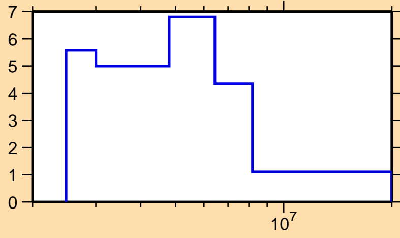
\Delta\sigma/\sigma vs. E for ^{100}\text{Zr}(n,n\text{onel.})
