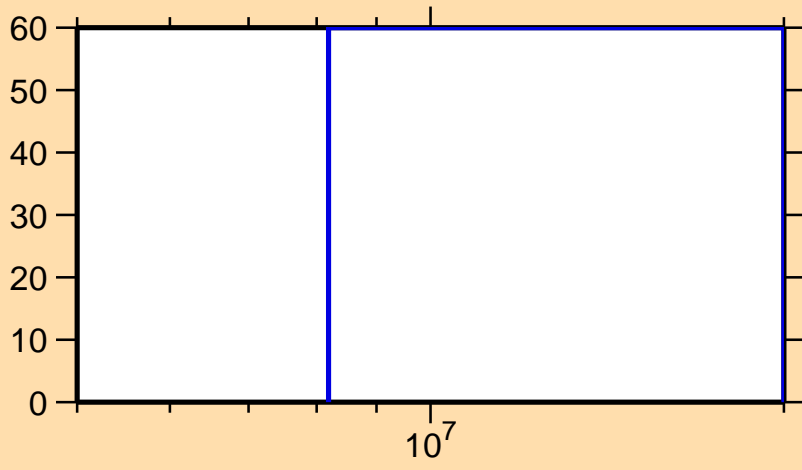
\Delta\sigma/\sigma vs. E for ^{100}\text{Zr}(n,\gamma)
