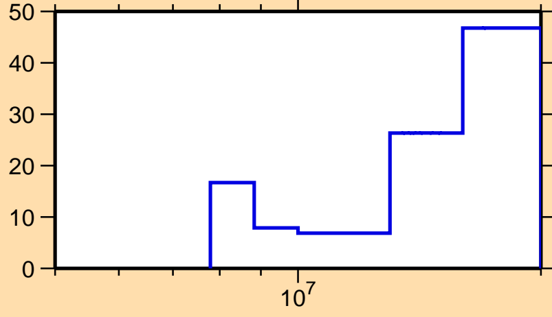
\Delta\sigma/\sigma vs. E for ^{101}\text{Zr}(n,2n)
