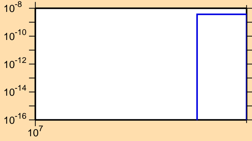
\sigma vs. E for ^{101}\text{Zr}(n,nt)
