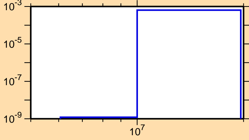
\sigma vs. E for ^{101}\text{Zr}(n,p)
