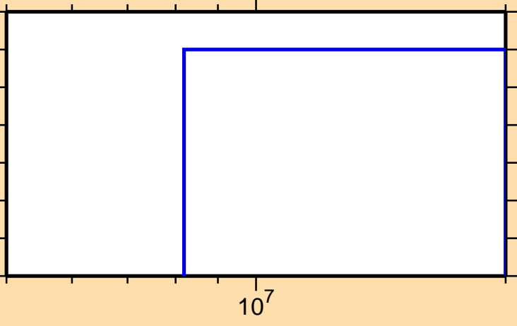
\sigma vs. E for ^{101}\text{Zr}(n,n\alpha)
