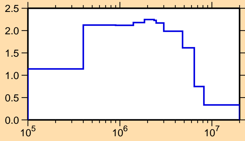
\sigma vs. E for ^{101}\text{Zr}(n,\text{inel.})
