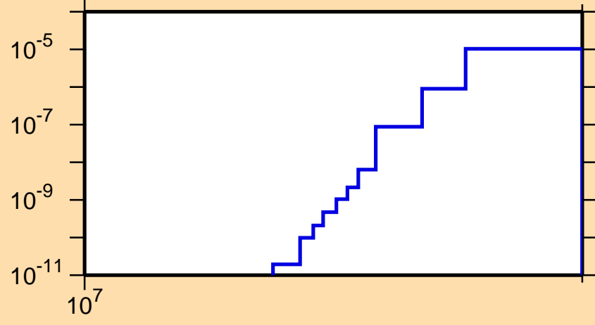
\sigma vs. E for ^{102}\text{Zr}(n,n\alpha)
