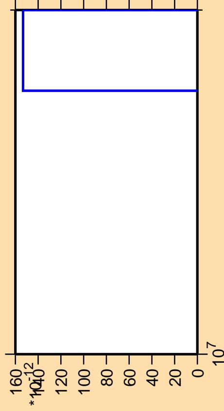
\Delta\sigma/\sigma vs. E for ^{102}\text{Zr}(n,2np)
