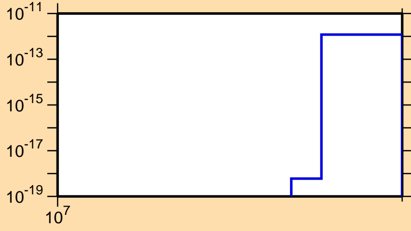
\sigma vs. E for ^{102}\text{Zr}(n,2n\alpha)
