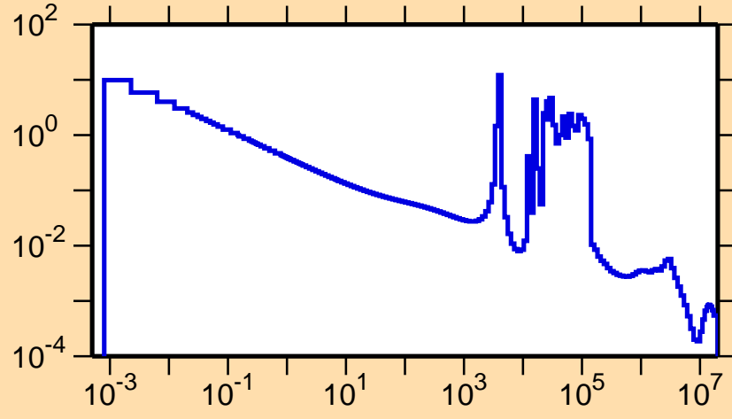
\sigma vs. E for ^{102}\text{Zr}(n,\gamma)
