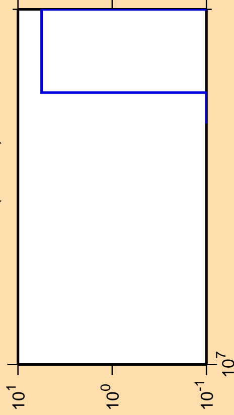
\Delta\sigma/\sigma vs. E for ^{102}\text{Zr}(n,2n\alpha)
