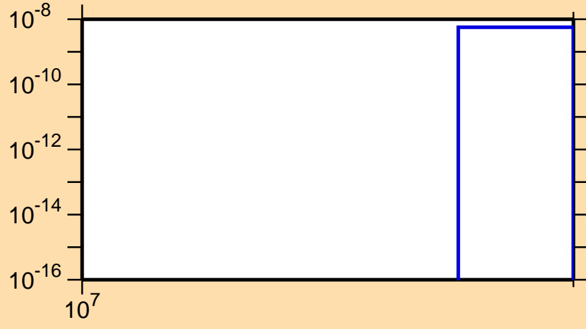
\sigma vs. E for ^{102}\text{Zr}(n,nt)
