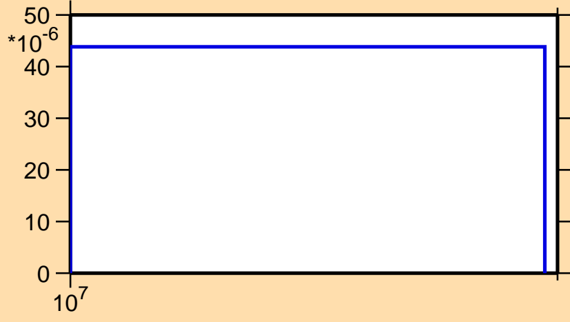
\sigma vs. E for ^{102}\text{Zr}(n,p)
