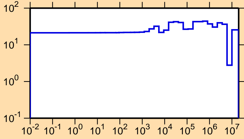
\Delta\sigma/\sigma vs. E for ^{102}\text{Zr}(n,\text{el.})
