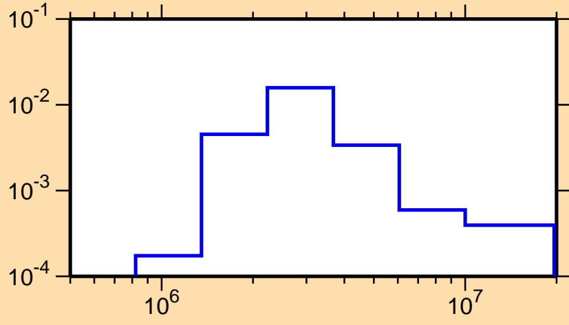
\sigma vs. E for ^{102}\text{Zr}(n,n_4)
