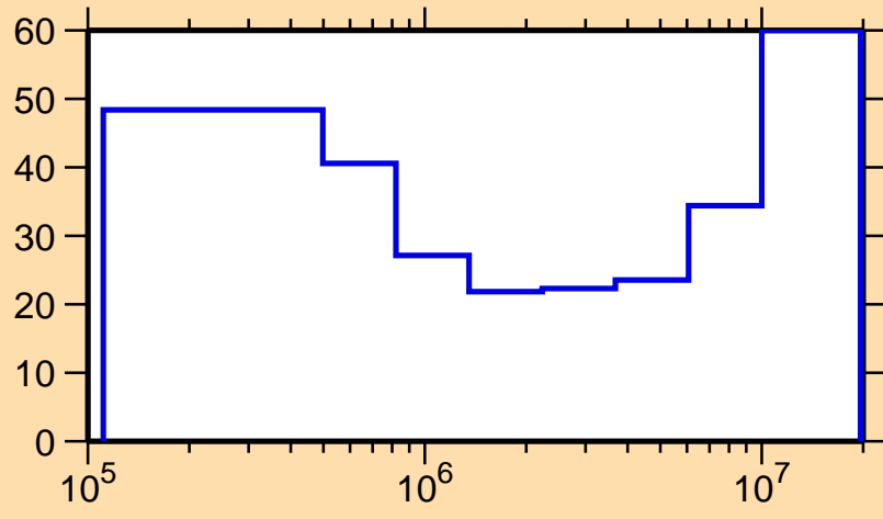
\Delta\sigma/\sigma vs. E for ^{102}\text{Zr}(n,\text{inel.})
