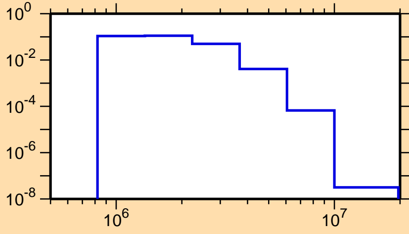
\sigma vs. E for ^{102}\text{Zr}(n,n_3)
