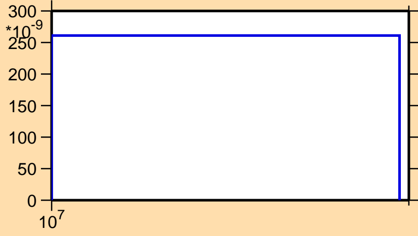
\sigma vs. E for ^{102}\text{Zr}(n,np)
