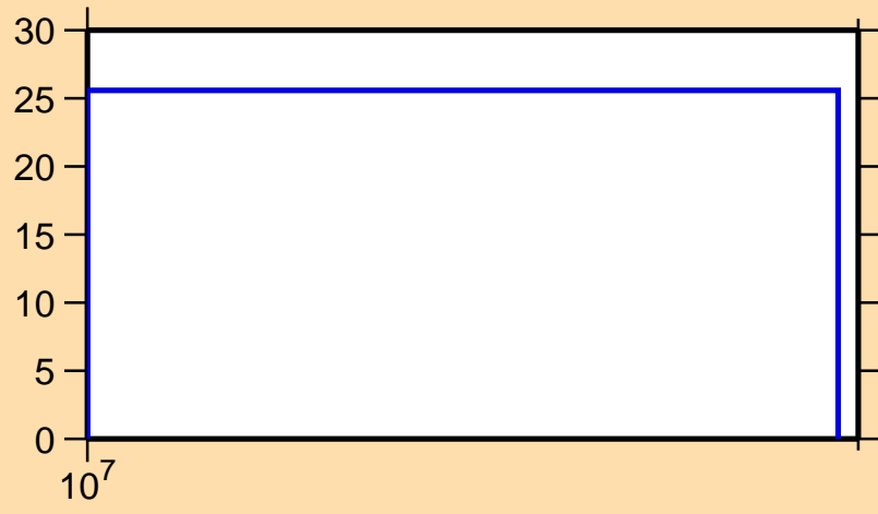
\Delta\sigma/\sigma vs. E for ^{102}\text{Zr}(n,\text{el.})
