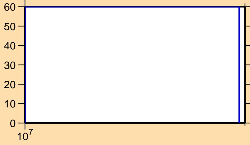
\Delta\sigma/\sigma vs. E for ^{102}\text{Zr}(n,n_1)
