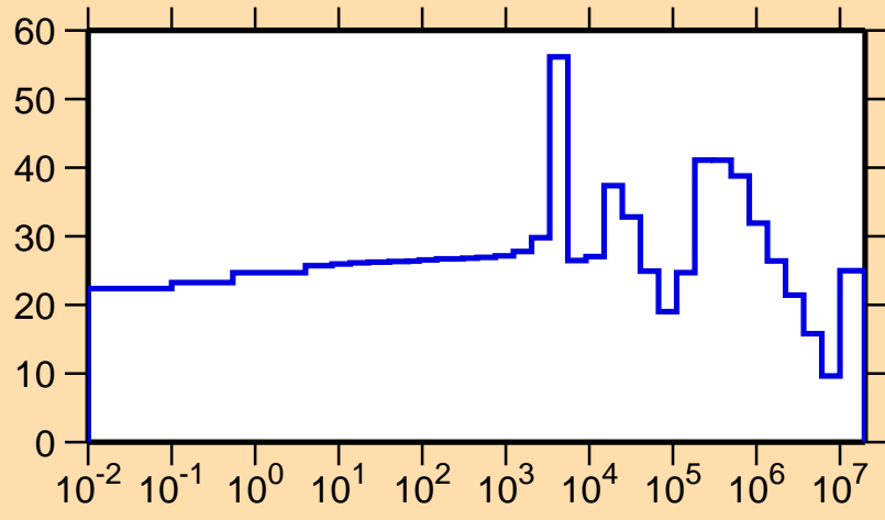
\Delta\sigma/\sigma vs. E for ^{102}\text{Zr}(n,\text{tot.})
