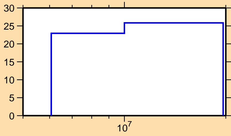
\Delta\sigma/\sigma vs. E for ^{102}\text{Zr}(n,\text{nonel.})
