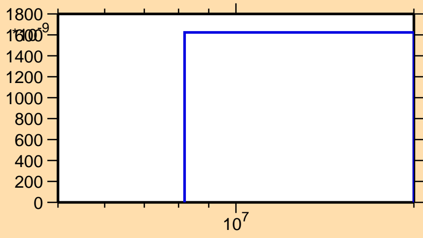
\sigma vs. E for ^{102}\text{Zr}(n,d)
