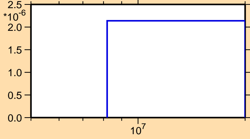
\sigma vs. E for ^{102}\text{Zr}(n,\alpha)
