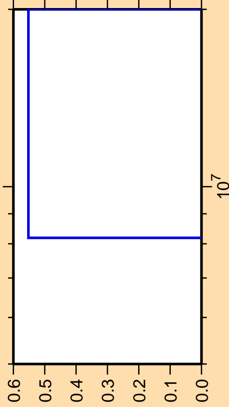
\Delta\sigma/\sigma vs. E for ^{102}\text{Zr}(n,nd)
