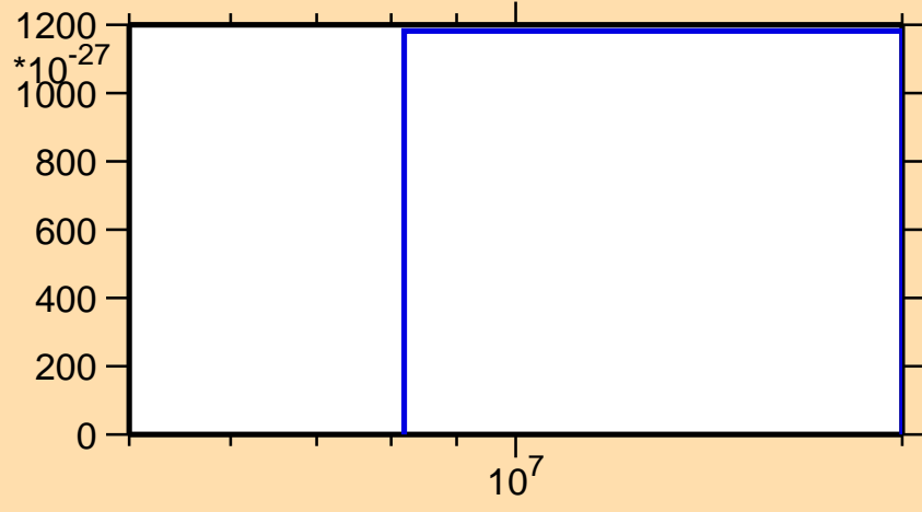
\sigma vs. E for ^{102}\text{Zr}(n,2np)
