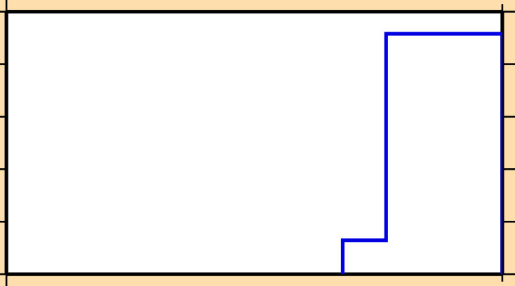
\sigma vs. E for ^{103}\text{Zr}(n,2n\alpha)
