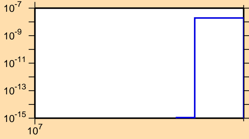
\sigma vs. E for ^{103}\text{Zr}(n,nt)
