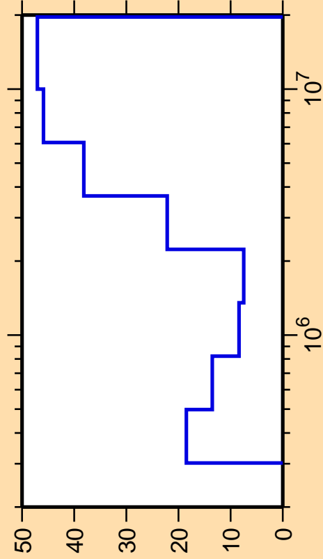
\Delta\sigma/\sigma vs. E for ^{103}\text{Zr}(n,n_4)
