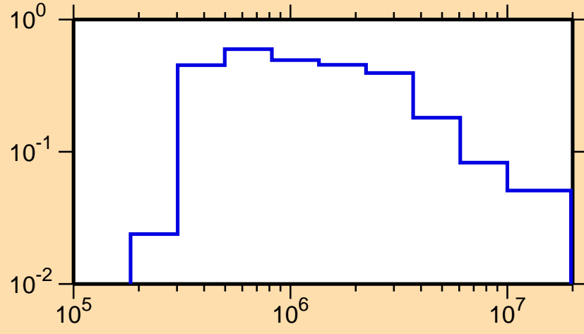
\sigma vs. E for ^{103}\text{Zr}(n,n_2)
