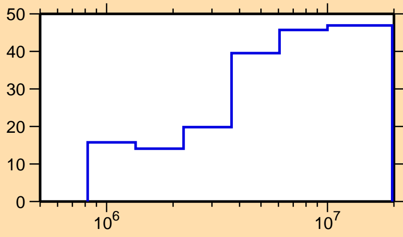
\Delta\sigma/\sigma vs. E for ^{103}\text{Zr}(n,n_1)
