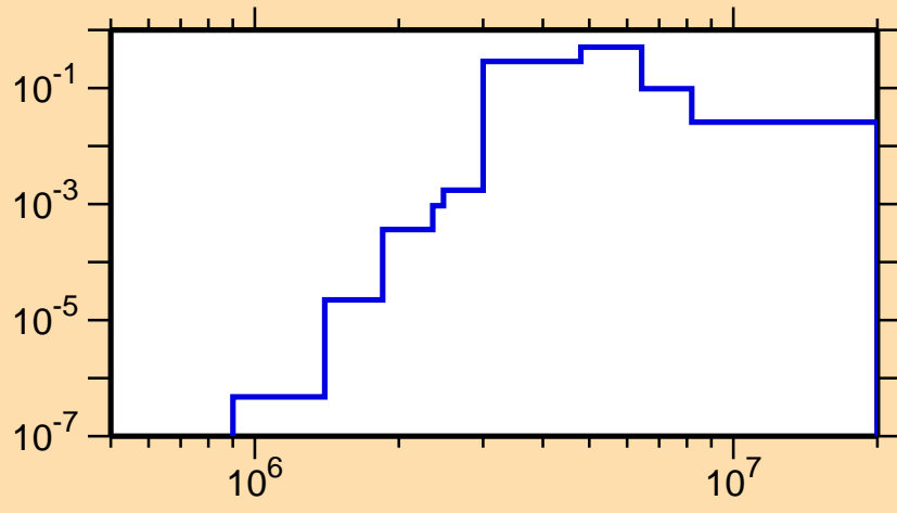
\sigma vs. E for ^{103}\text{Zr}(n,n\text{cont.})
