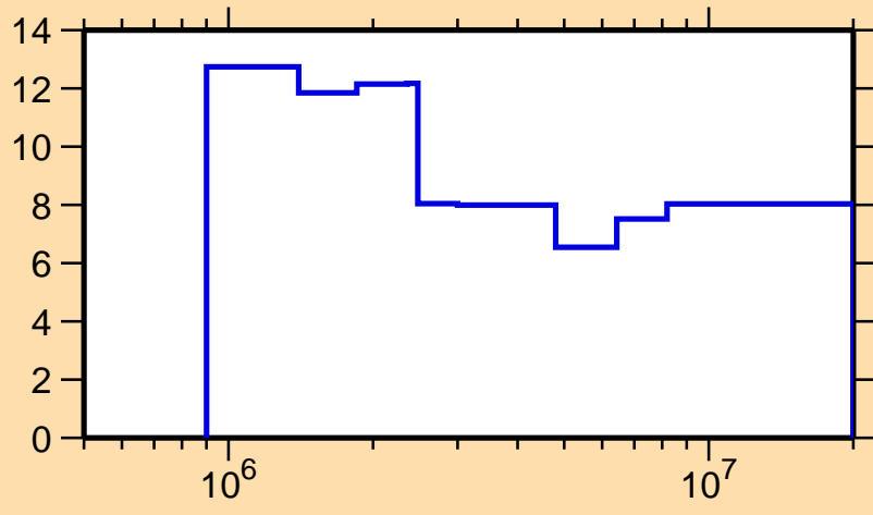
\Delta\sigma/\sigma vs. E for ^{103}\text{Zr}(n,nonel.)
