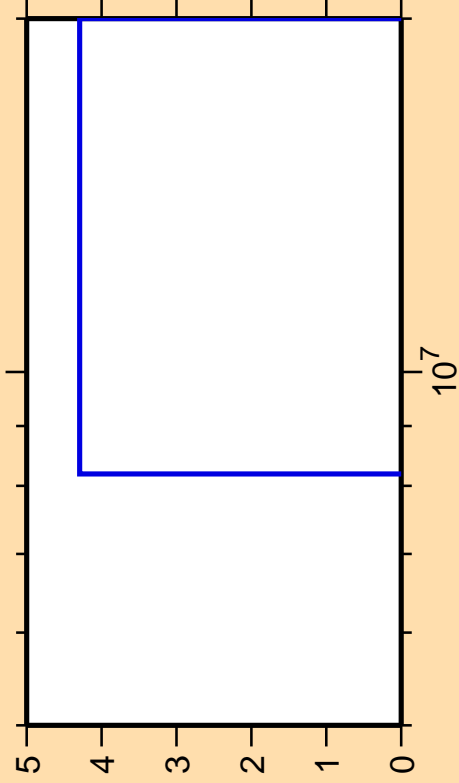
\Delta\sigma/\sigma vs. E for ^{103}\text{Zr}(n,2n\alpha)
