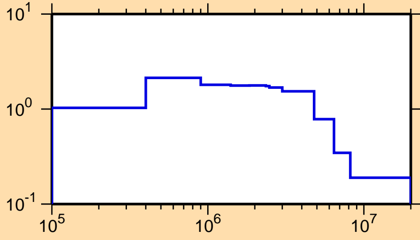
\sigma vs. E for ^{103}\text{Zr}(n,\text{inel.})
