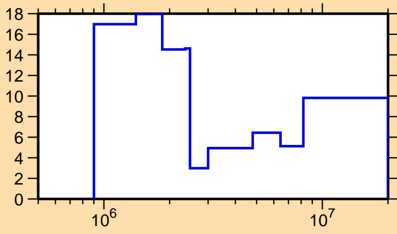
\Delta\sigma/\sigma vs. E for ^{103}\text{Zr}(n, el.)
