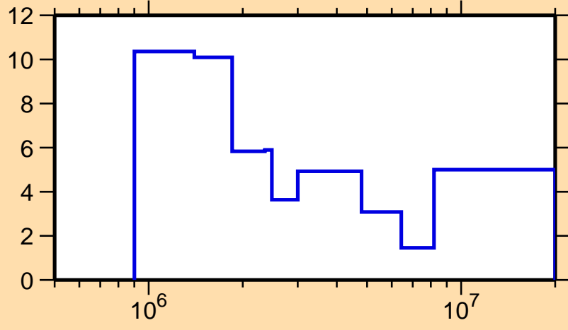
\Delta\sigma/\sigma vs. E for ^{103}\text{Zr}(n,tot.)
