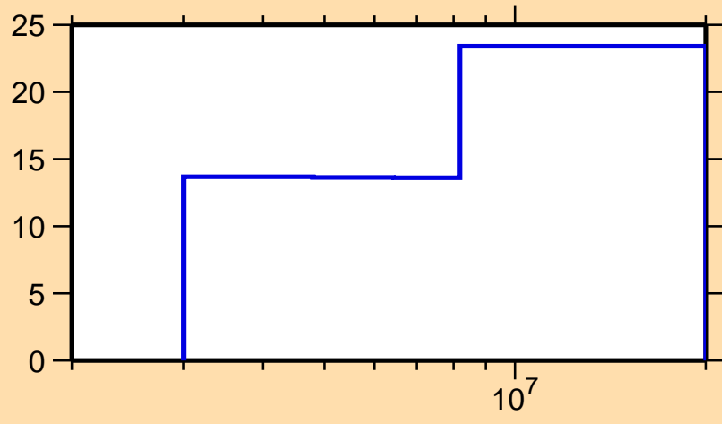
\Delta\sigma/\sigma vs. E for ^{103}\text{Zr}(n,2n)
