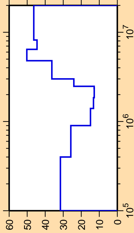
\Delta\sigma/\sigma vs. E for ^{103}\text{Zr}(n,n_2)
