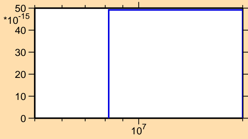
\sigma vs. E for ^{103}\text{Zr}(n,2np)
