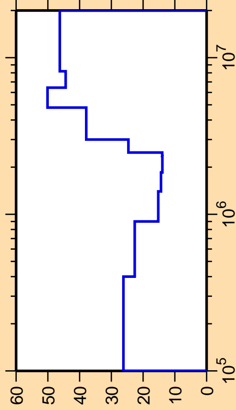
\Delta\sigma/\sigma vs. E for ^{103}\text{Zr}(n,n_1)
