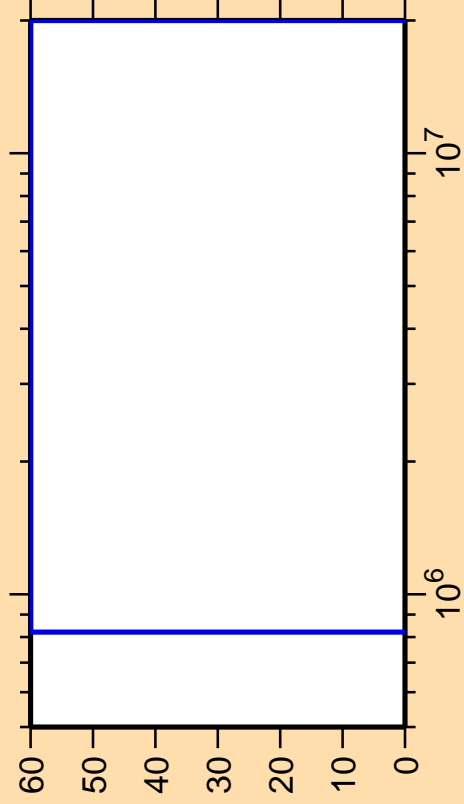
\Delta\sigma/\sigma vs. E for ^{95}\text{Ag}(n,n_3)
