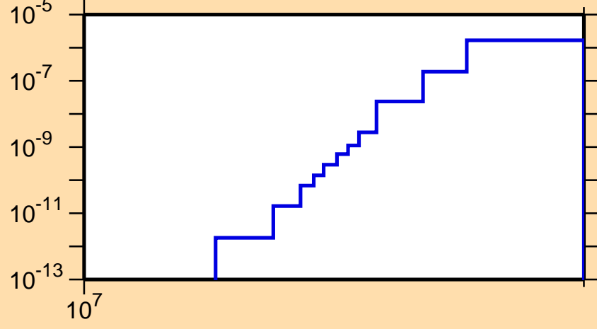
\sigma vs. E for ^{95}\text{Ag}(\text{mt } 45)
