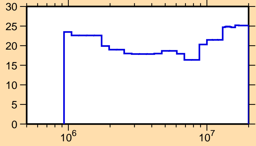
\Delta\sigma/\sigma vs. E for ^{95}\text{Ag}(n,n\text{nonel.})
