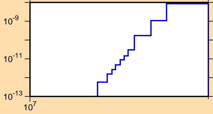
\sigma vs. E for ^{95}\text{Ag}(\text{mt117})
