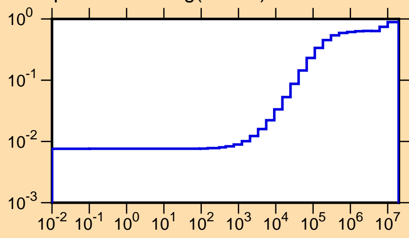
\mu vs. E for ^{95}\text{Ag}(\text{mt251})
