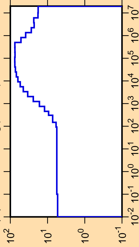
\Delta\mu/\mu vs. E for ^{95}\text{Ag}(\text{mt251})
