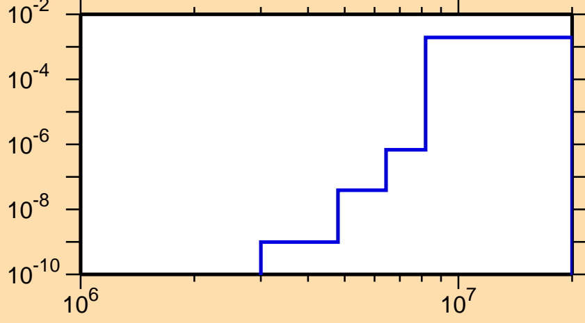
\sigma vs. E for ^{95}\text{Ag}(n,\text{He3})
