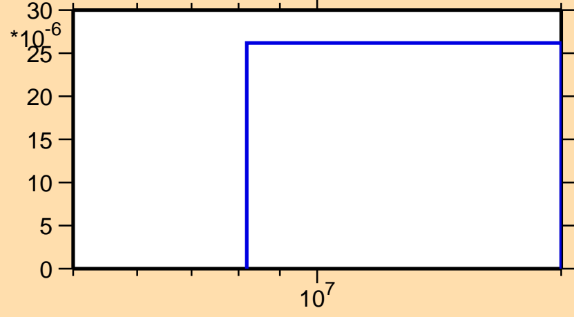
\sigma vs. E for ^{95}\text{Ag}(n,t)
