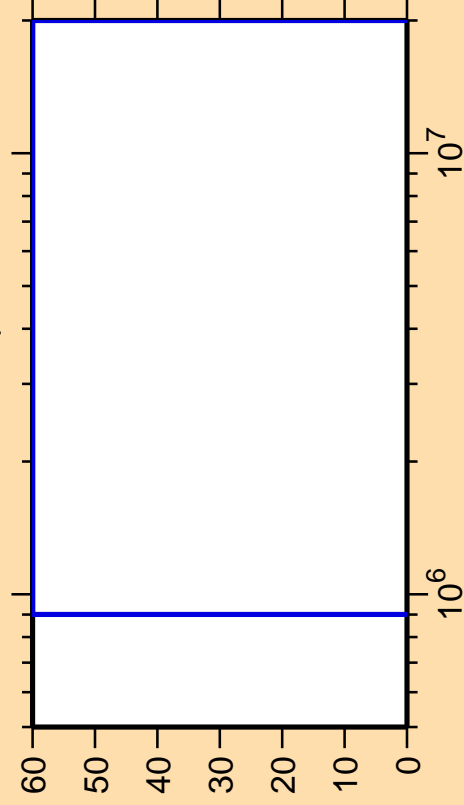
\Delta\sigma/\sigma vs. E for ^{95}\text{Ag}(n,n_4)
