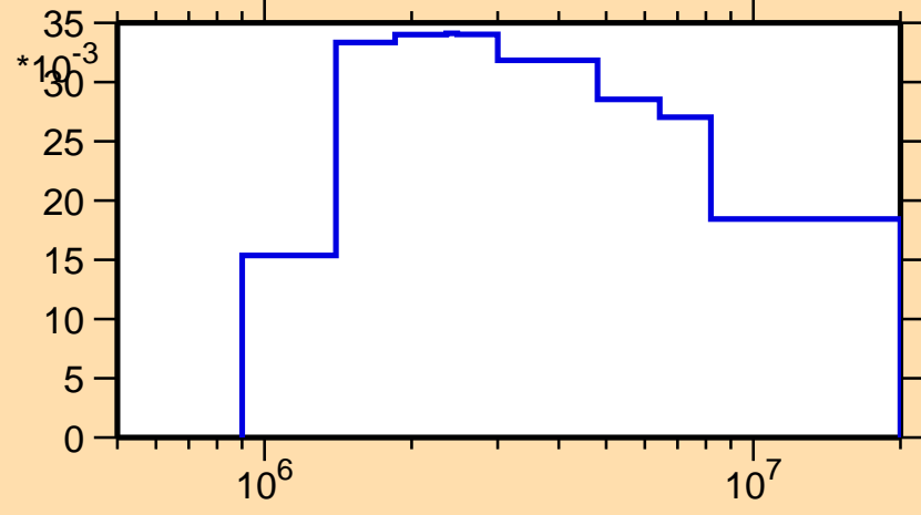
\sigma vs. E for ^{95}\text{Ag}(n,n_4)
