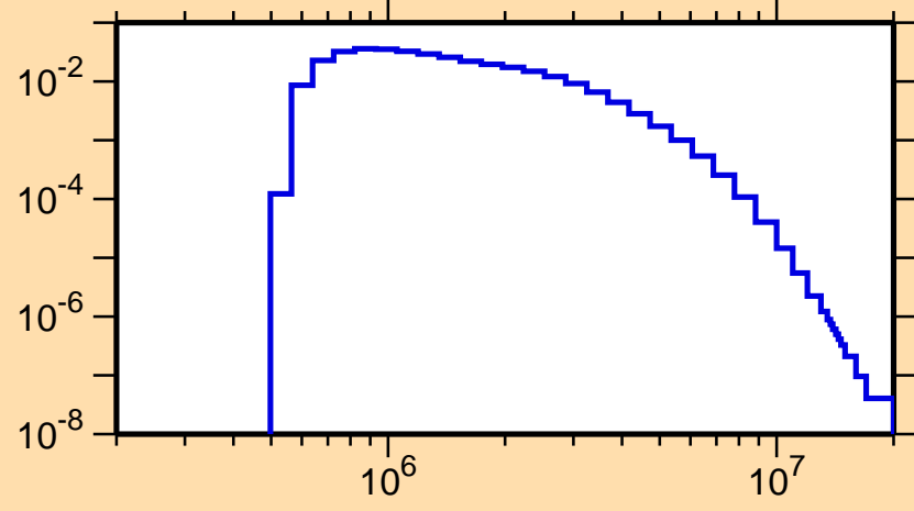
\sigma vs. E for ^{96}\text{Ag}(n,n_3)
