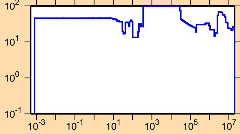
\Delta\sigma/\sigma vs. E for ^{96}\text{Ag}(n,\text{el.})
