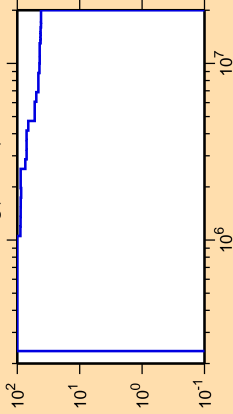
\Delta\sigma/\sigma vs. E for ^{96}\text{Ag}(n,\text{inel.})
