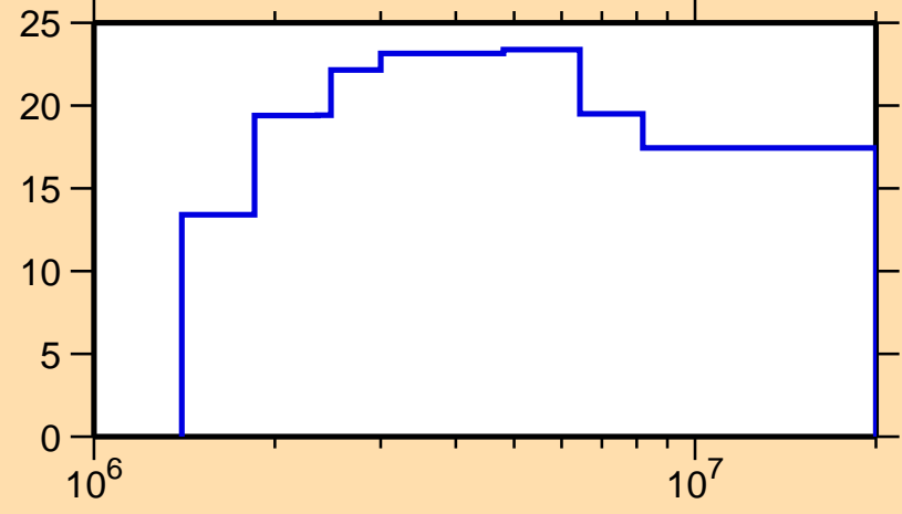
\Delta\sigma/\sigma vs. E for ^{96}\text{Ag}(n,n\text{nonel.})
