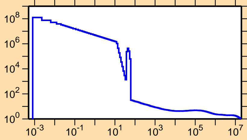
\sigma vs. E for ^{96}\text{Ag}(n,\text{nonel.})
