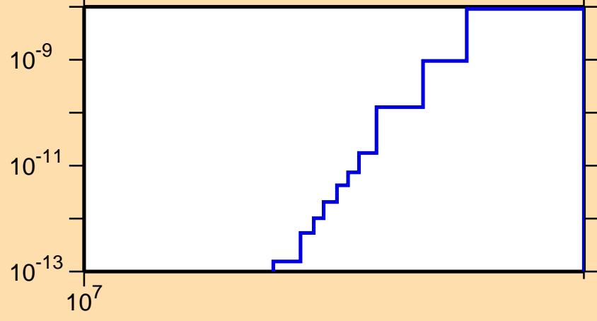
\sigma vs. E for ^{96}\text{Ag}(\text{mt117})
