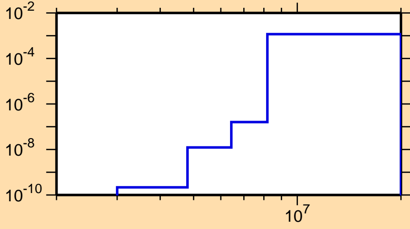
\sigma vs. E for ^{96}\text{Ag}(n,\text{He3})
