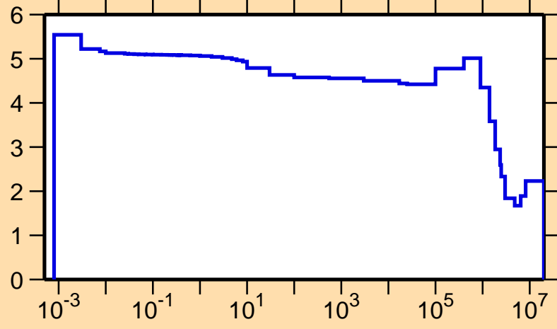
\sigma vs. E for ^{96}\text{Ag}(n,\text{el.})
