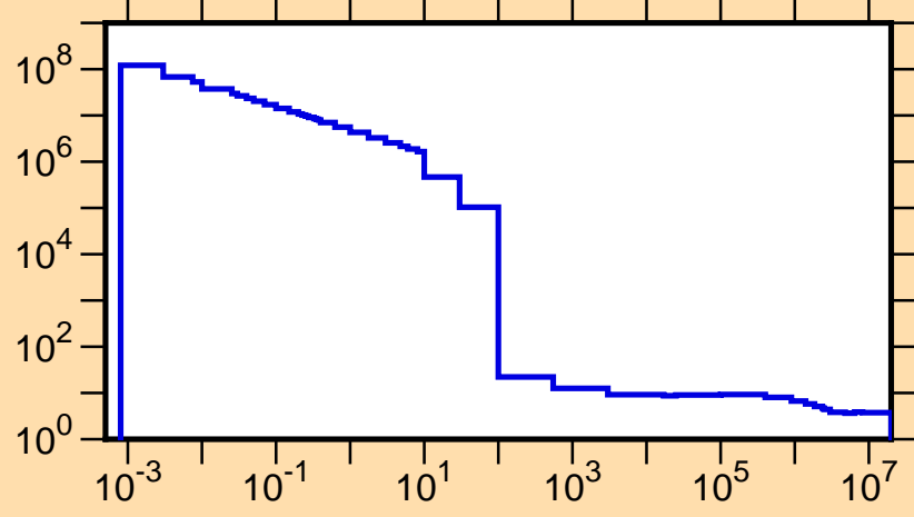
\sigma vs. E for ^{96}\text{Ag}(n,\text{tot.})
