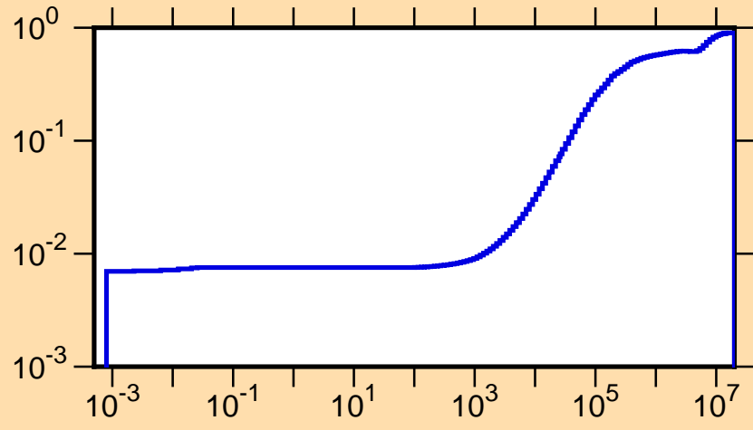
\mu vs. E for ^{97}\text{Ag}(\text{mt251})
