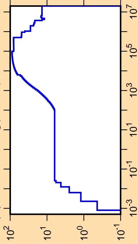
\Delta\mu/\mu vs. E for ^{97}\text{Ag}(\text{mt251})
