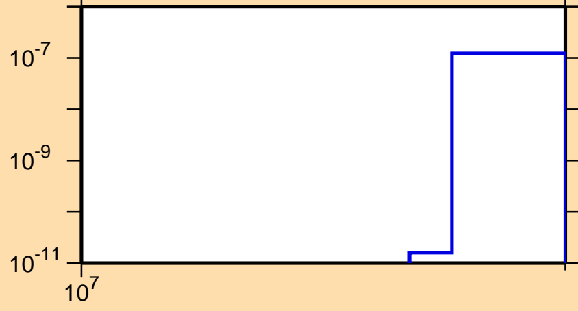
\sigma vs. E for ^{97}\text{Ag}(n,\text{pt})
