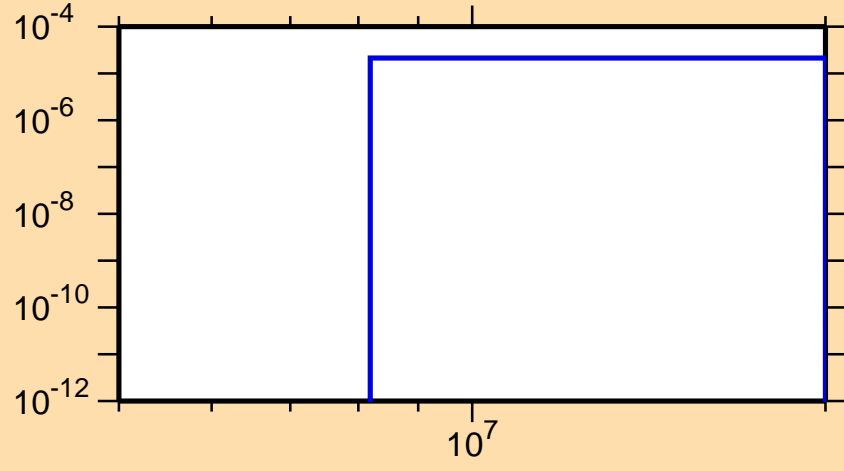
\sigma vs. E for ^{97}\text{Ag}(n,t)
