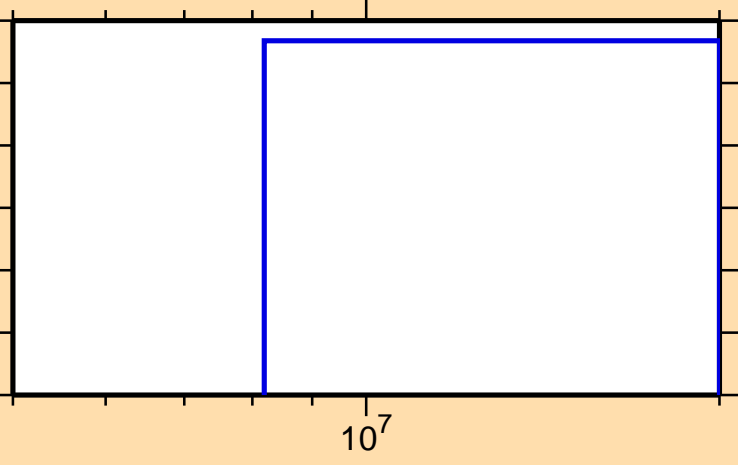
\sigma vs. E for ^{97}\text{Ag}(n,\text{nd})
