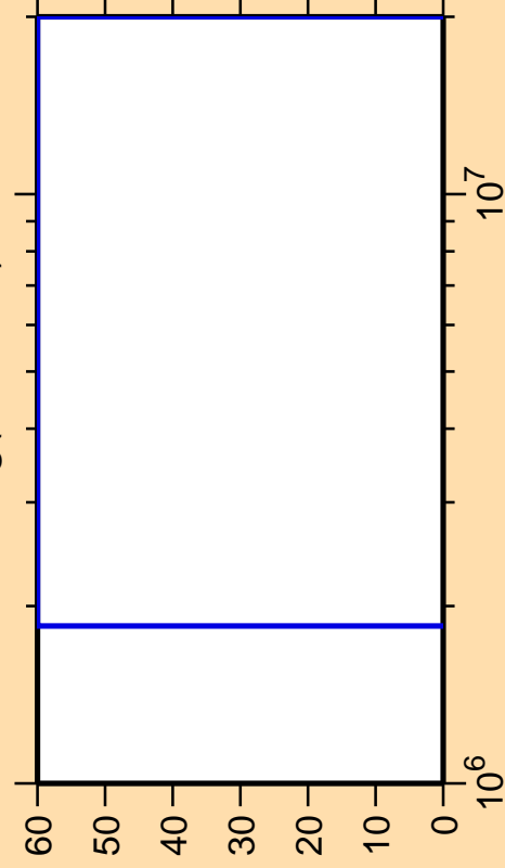
\Delta\sigma/\sigma vs. E for ^{97}\text{Ag}(n,n\text{cont.})
