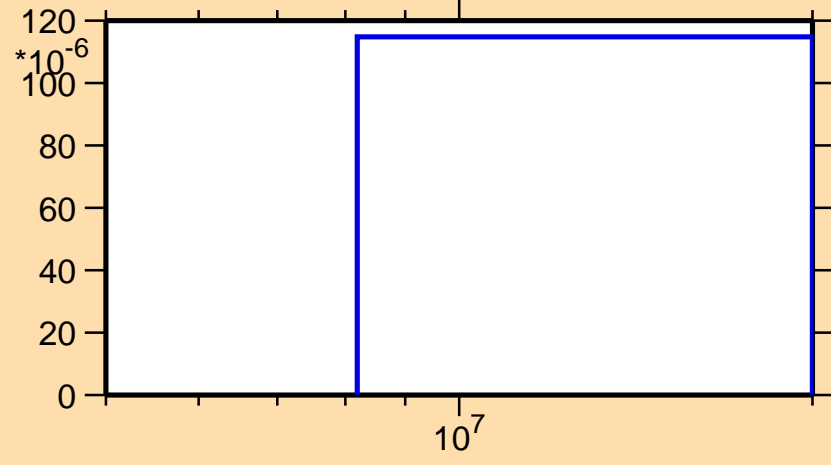
\sigma vs. E for ^{97}\text{Ag}(n,2n)
