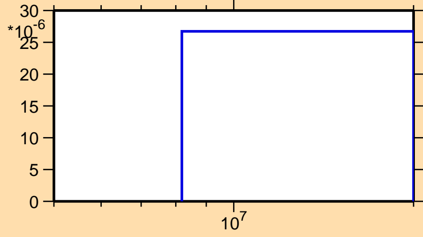
\sigma vs. E for ^{97}\text{Ag}(n,n\alpha)
