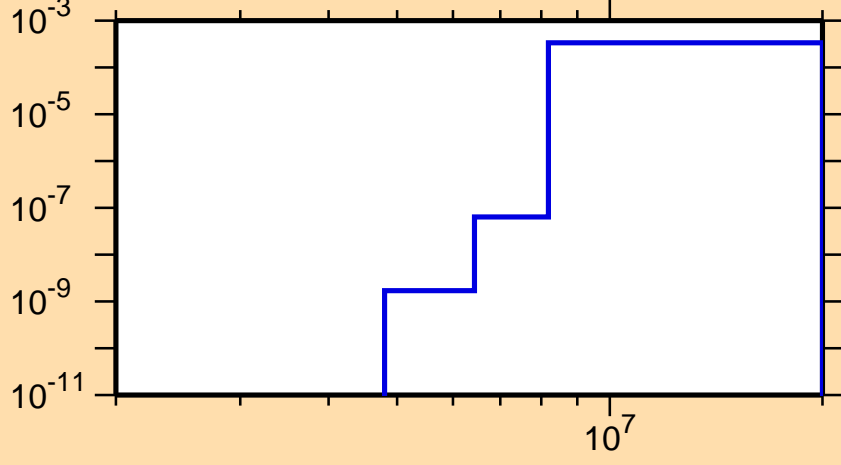
\sigma vs. E for ^{97}\text{Ag}(n,\text{He3})
