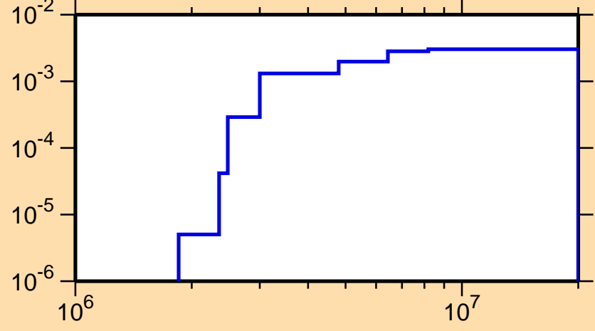
\sigma vs. E for ^{97}\text{Ag}(n,n\text{cont.})
