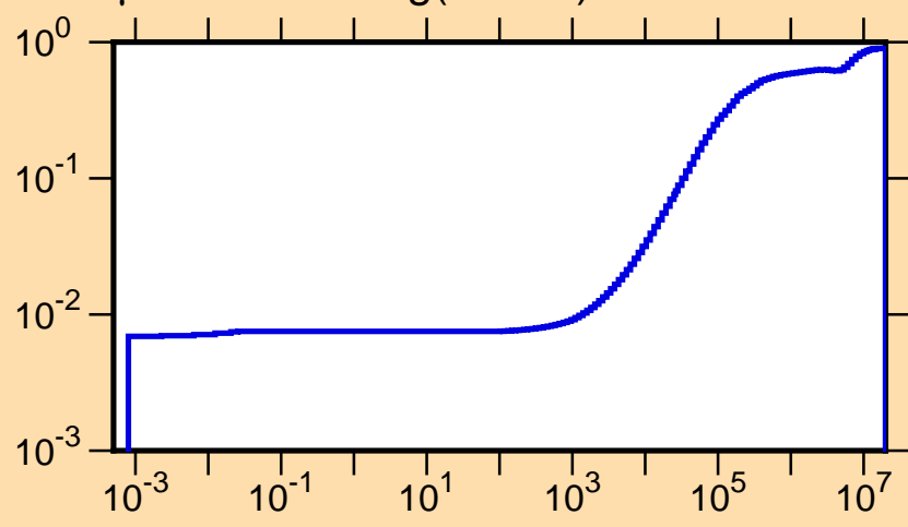
\mu vs. E for ^{98}\text{Ag}(\text{mt251})
