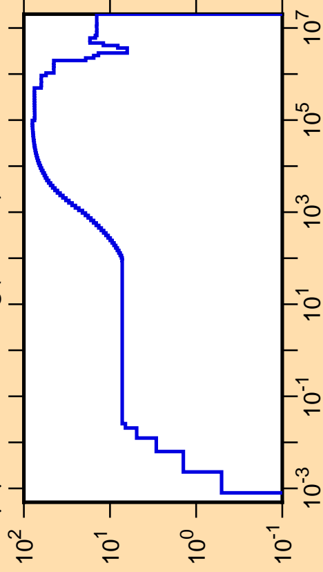
\Delta\mu/\mu vs. E for ^{98}\text{Ag}(\text{mt251})
