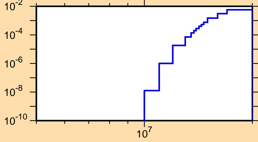
\sigma vs. E for ^{98}\text{Ag}(n,\text{pd})
