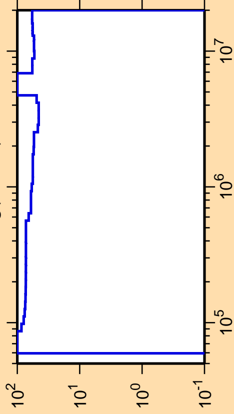
\Delta\sigma/\sigma vs. E for ^{98}\text{Ag}(n,\text{inel.})
