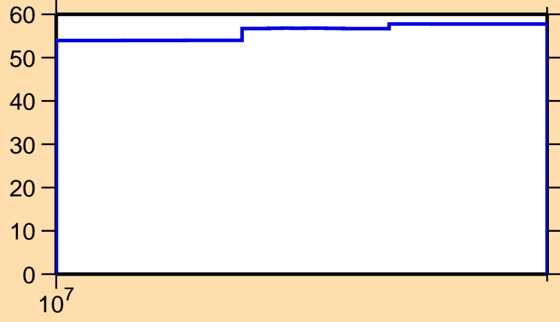
\Delta\sigma/\sigma vs. E for ^{98}\text{Ag}(n,\text{inel.})
