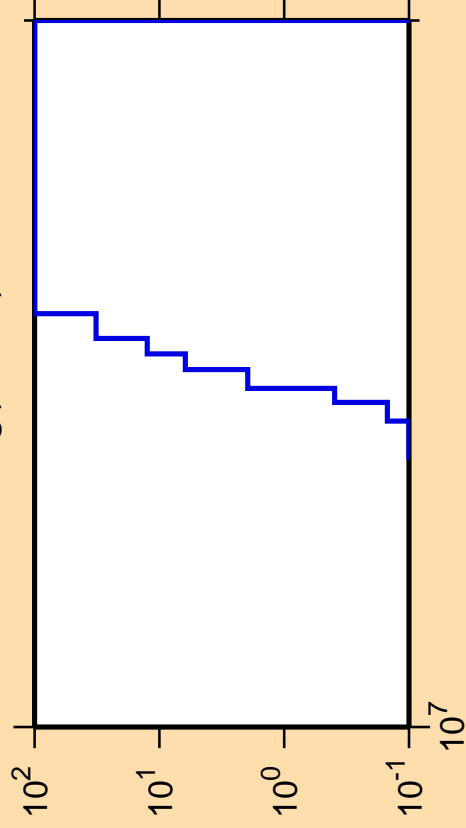
\Delta\sigma/\sigma vs. E for ^{98}\text{Ag}(\text{mt } 34)
