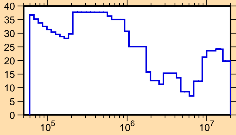
\Delta\sigma/\sigma vs. E for ^{98}\text{Ag}(n,\text{tot.})
