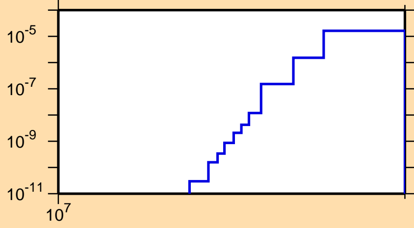
\sigma vs. E for ^{98}\text{Ag}(\text{mt } 45)
