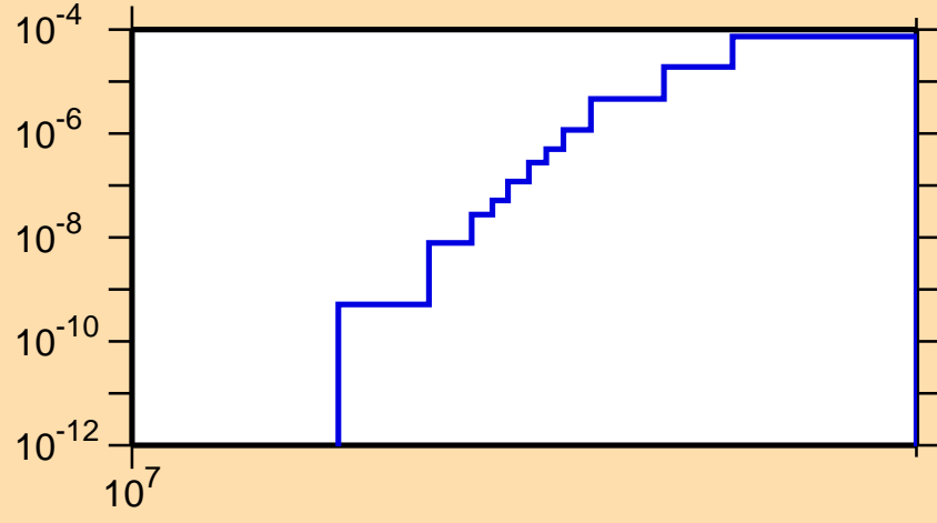
\sigma vs. E for ^{98}\text{Ag}(n,\text{nd})
