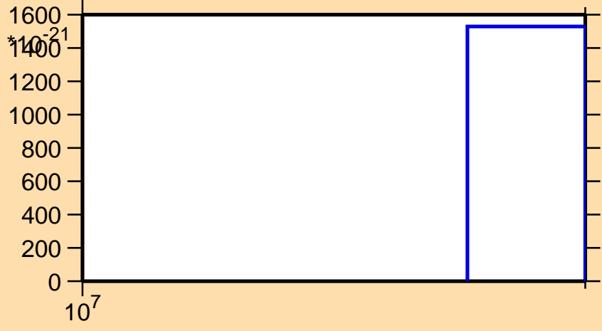
\sigma vs. E for ^{98}\text{Ag}(n,nt)
