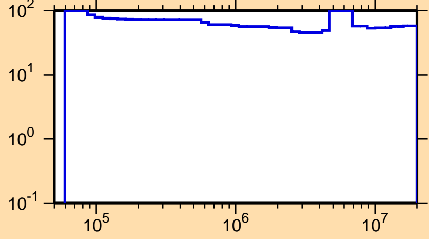
\Delta\sigma/\sigma vs. E for ^{98}\text{Ag}(n,\text{inel.})
