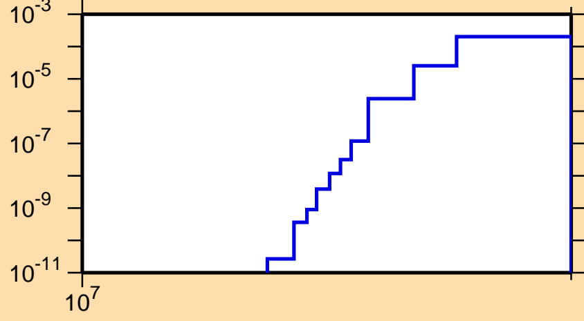
\sigma vs. E for ^{98}\text{Ag}(n,\text{pt})
