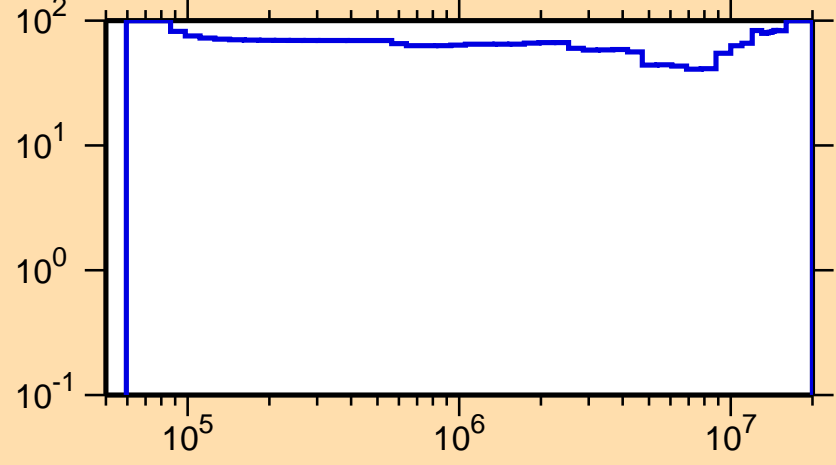
\Delta\sigma/\sigma vs. E for ^{98}\text{Ag}(n,n_1)
