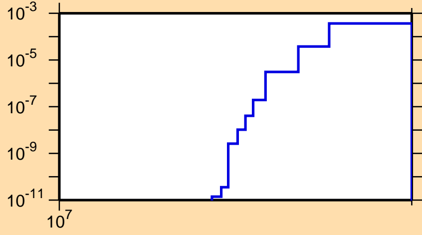
\sigma vs. E for ^{98}\text{Ag}(n,2np)
