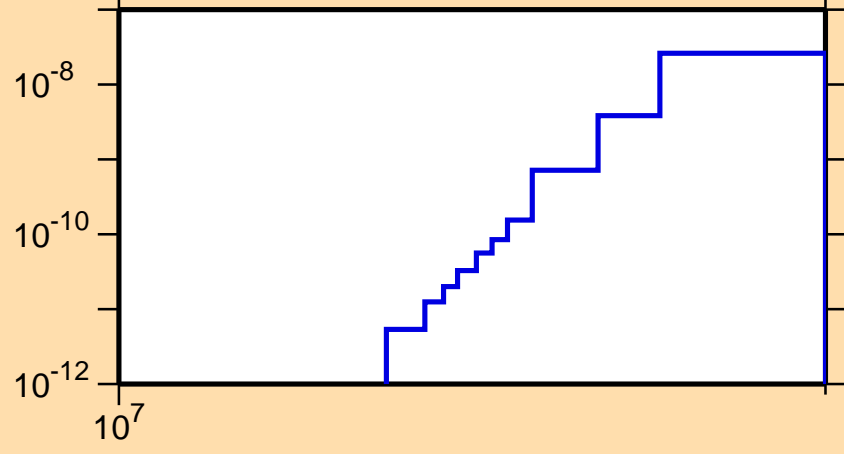
\sigma vs. E for ^{98}\text{Ag}(\text{mt117})
