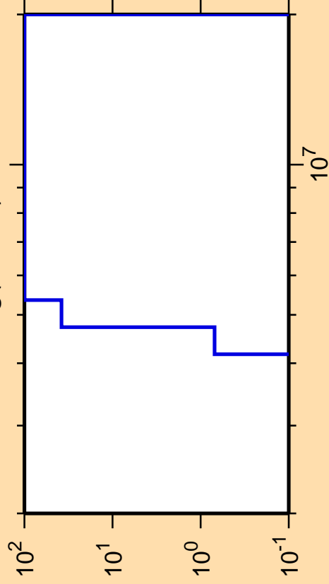
\Delta\sigma/\sigma vs. E for ^{98}\text{Ag}(n,\text{He3})
