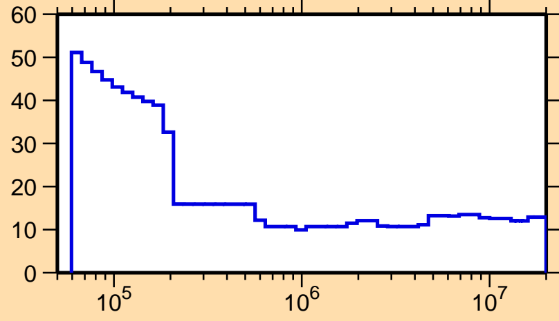
\Delta\sigma/\sigma vs. E for ^{98}\text{Ag}(n,\text{nonel.})
