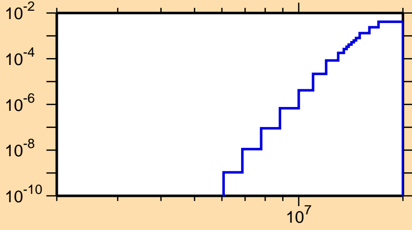
\sigma vs. E for ^{98}\text{Ag}(n,\text{He3})
