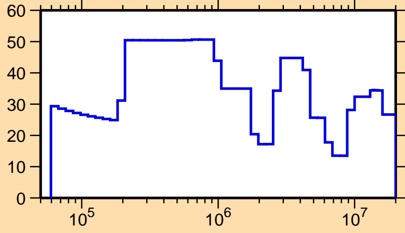
\Delta\sigma/\sigma vs. E for ^{98}\text{Ag}(n,\text{el.})
