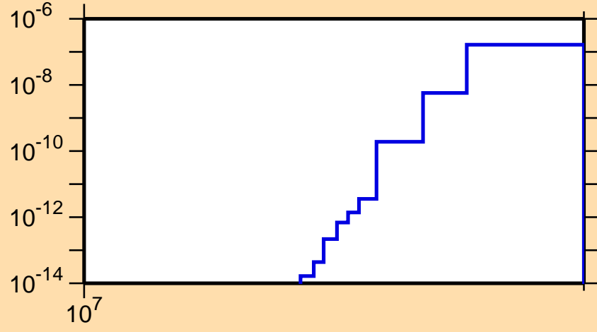
\sigma vs. E for ^{98}\text{Ag}(\text{mt } 34)
