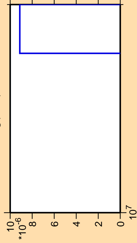
\Delta\sigma/\sigma vs. E for ^{98}\text{Ag}(n,nt)
