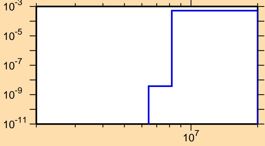
\sigma vs. E for ^{98}\text{Ag}(n,t)
