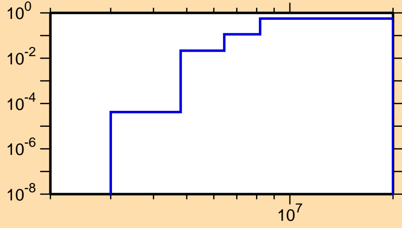
\sigma vs. E for ^{98}\text{Ag}(n,np)
