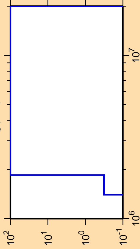
\Delta\sigma/\sigma vs. E for ^{98}\text{Ag}(n,d)
