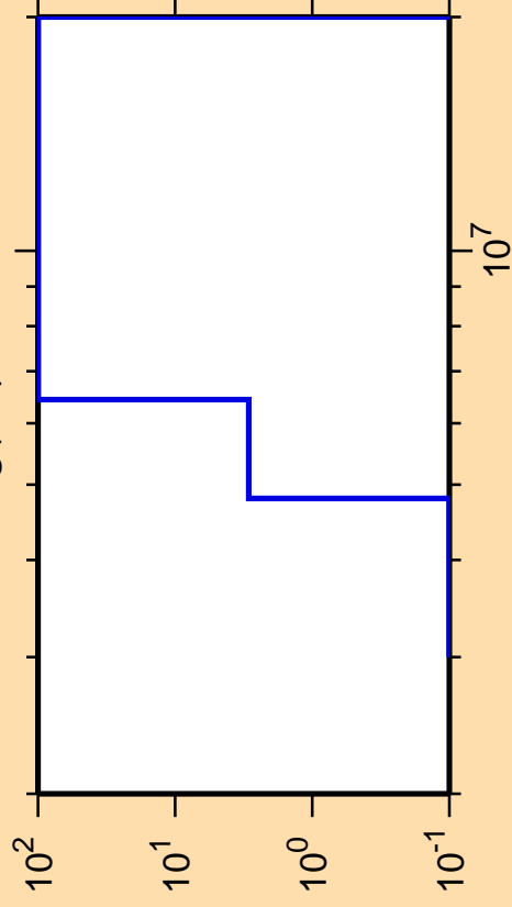
\Delta\sigma/\sigma vs. E for ^{98}\text{Ag}(n,t)
