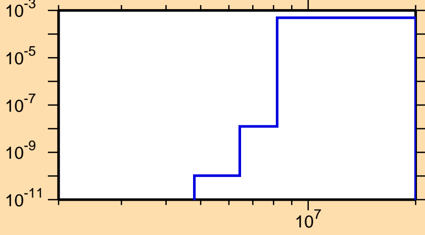
\sigma vs. E for ^{98}\text{Ag}(n,\text{He3})
