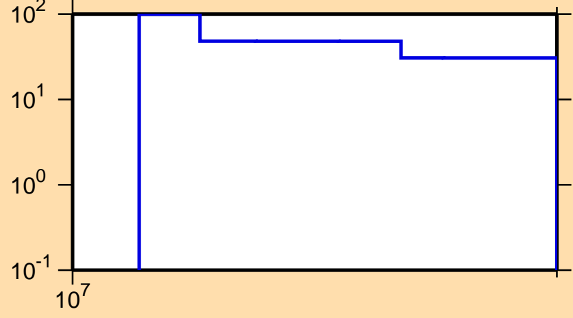
\Delta\sigma/\sigma vs. E for ^{99}\text{Ag}(n,2n)
