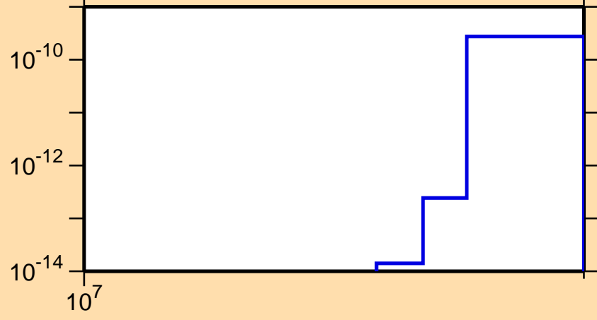
\sigma vs. E for ^{99}\text{Ag}(n,nt)
