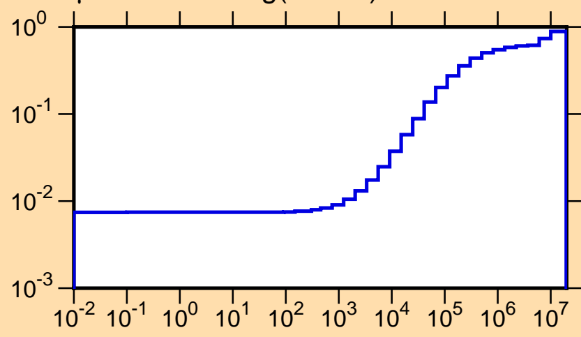
\mu vs. E for ^{99}\text{Ag}(\text{mt251})
