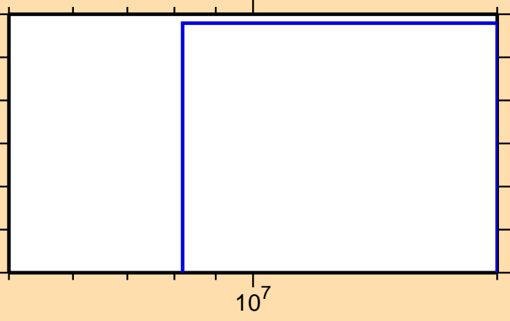
\sigma vs. E for ^{99}\text{Ag}(\text{mt117})
