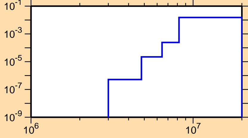
\sigma vs. E for ^{99}\text{Ag}(n,d)
