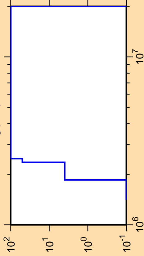
\Delta\sigma/\sigma vs. E for ^{99}\text{Ag}(n,d)
