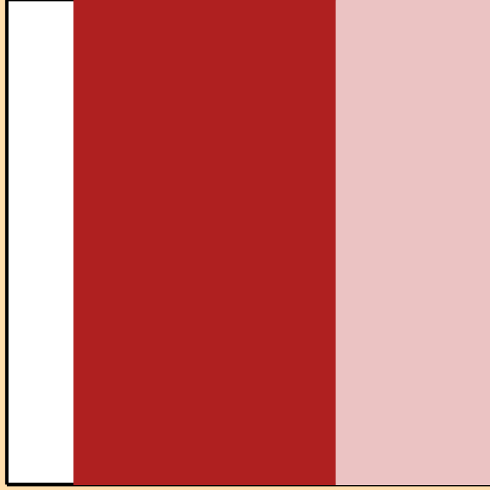
\Delta\sigma/\sigma vs. E for ^{99}\text{Ag}(n,2n)
