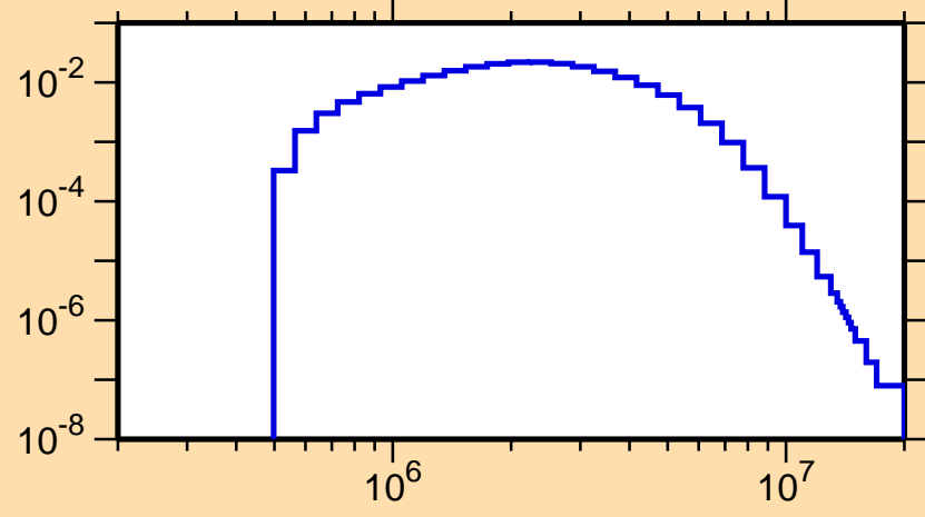
\sigma vs. E for ^{99}\text{Ag}(n,n_4)
