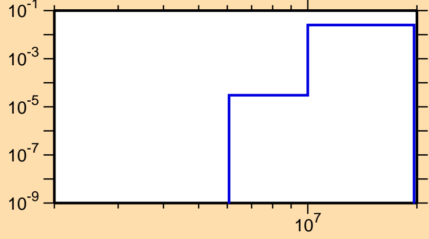
\sigma vs. E for ^{99}\text{Ag}(n,n\alpha)
