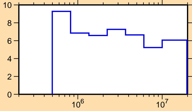
\Delta\sigma/\sigma vs. E for ^{99}\text{Ag}(n,n\text{nonel.})
