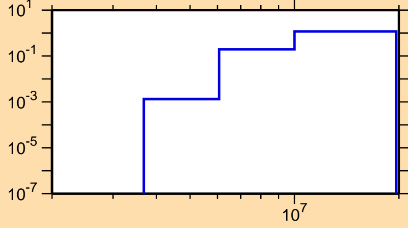
\sigma vs. E for ^{99}\text{Ag}(n,np)
