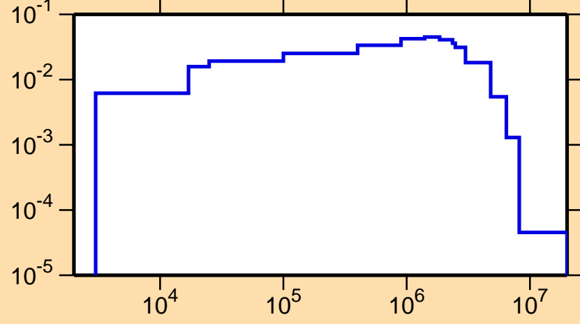
\sigma vs. E for ^{99}\text{Ag}(n,n_1)
