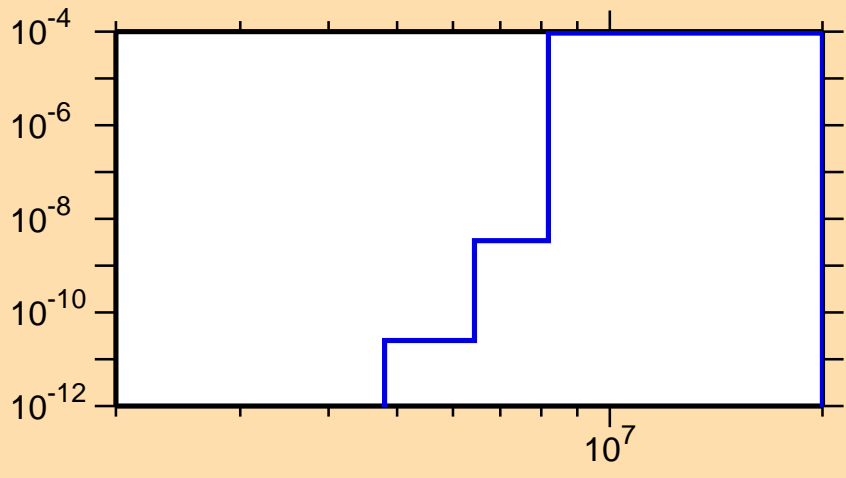
\sigma vs. E for ^{99}\text{Ag}(n,\text{He3})
