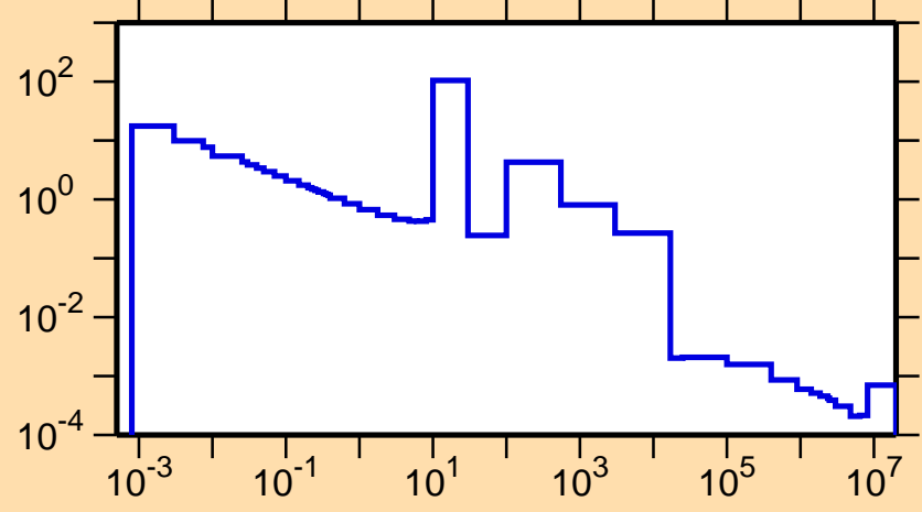
\sigma vs. E for ^{99}\text{Ag}(n,\gamma)
