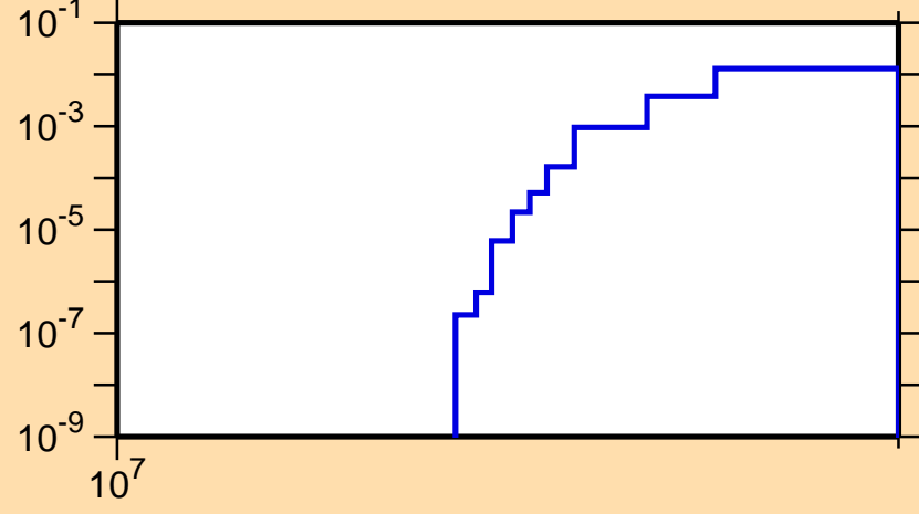
\sigma vs. E for ^{100}\text{Ag}(n,2np)
