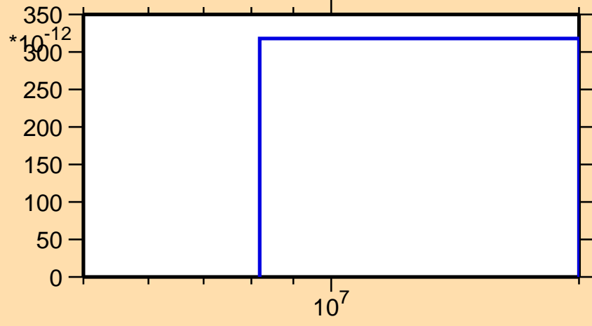
\sigma vs. E for ^{100}\text{Ag}(\text{mt } 34)
