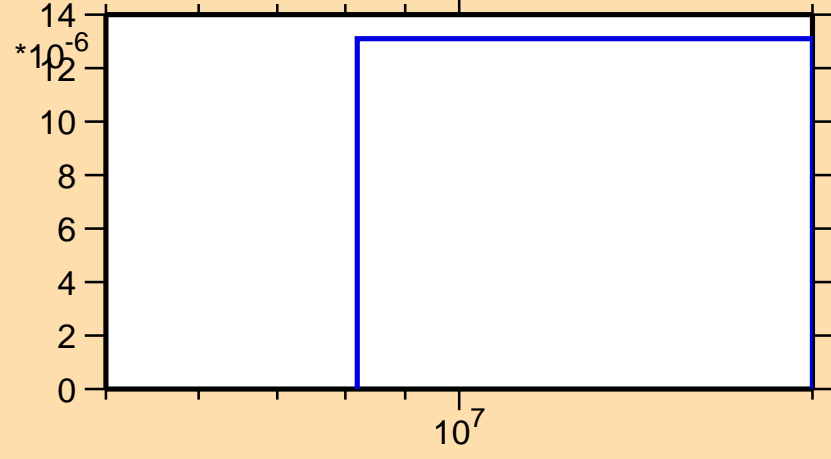
\sigma vs. E for ^{100}\text{Ag}(n,\text{pd})
