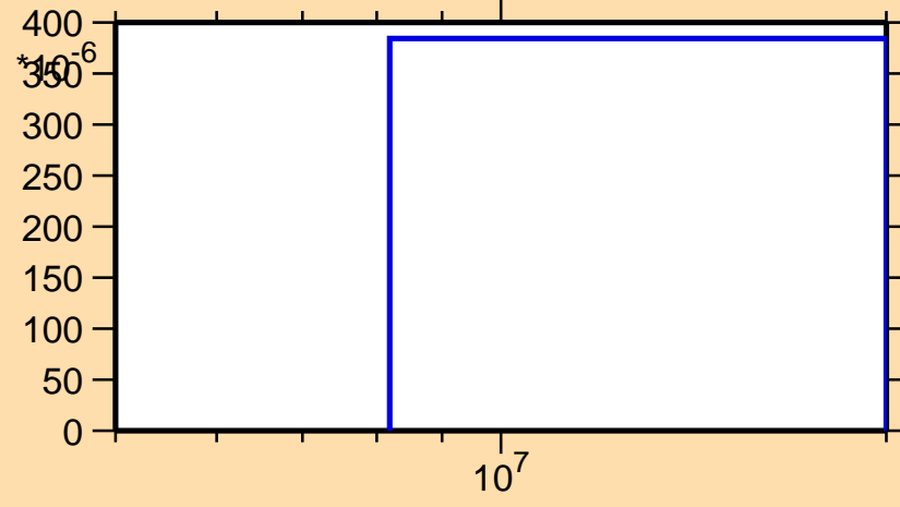
\sigma vs. E for ^{100}\text{Ag}(n,2np)
