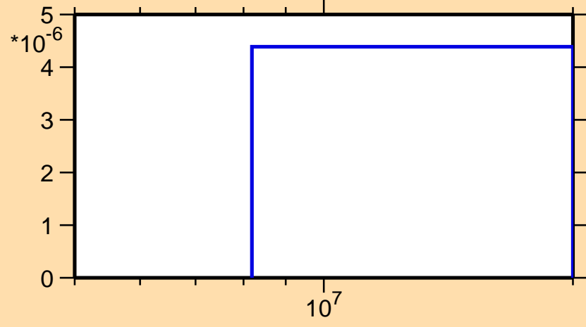
\sigma vs. E for ^{100}\text{Ag}(\text{mt } 45)
