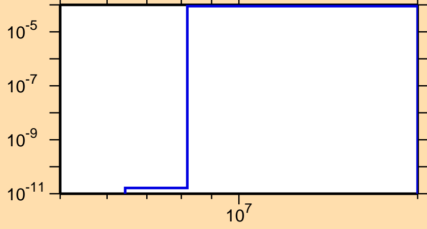
\sigma vs. E for ^{100}\text{Ag}(n,\text{He}3)
