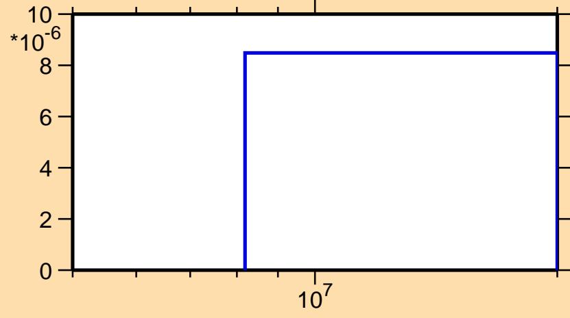
\sigma vs. E for ^{100}\text{Ag}(n,\text{nd})
