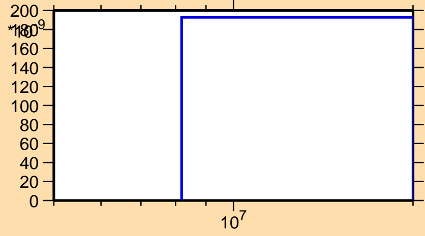
\sigma vs. E for ^{100}\text{Ag}(n,\text{pt})
