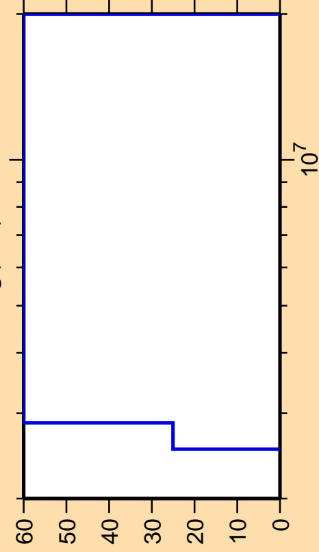
\Delta\sigma/\sigma vs. E for ^{100}\text{Ag}(n,d)
