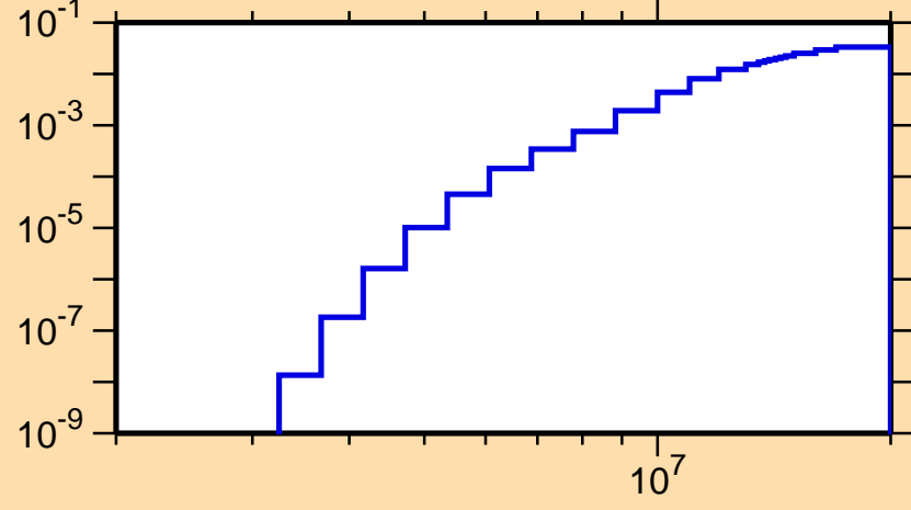
\sigma vs. E for ^{100}\text{Ag}(n,d)
