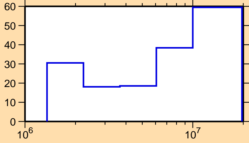
\Delta\sigma/\sigma vs. E for ^{100}\text{Ag}(n,ncont.)
