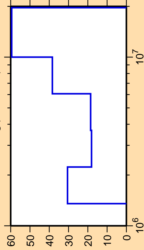
\Delta\sigma/\sigma vs. E for ^{100}\text{Ag}(n,n\text{cont.})
