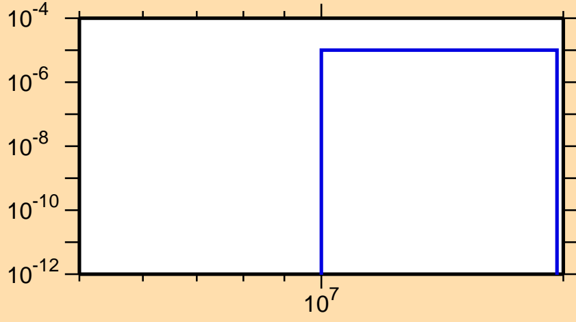
\sigma vs. E for ^{100}\text{Ag}(\text{mt } 45)
