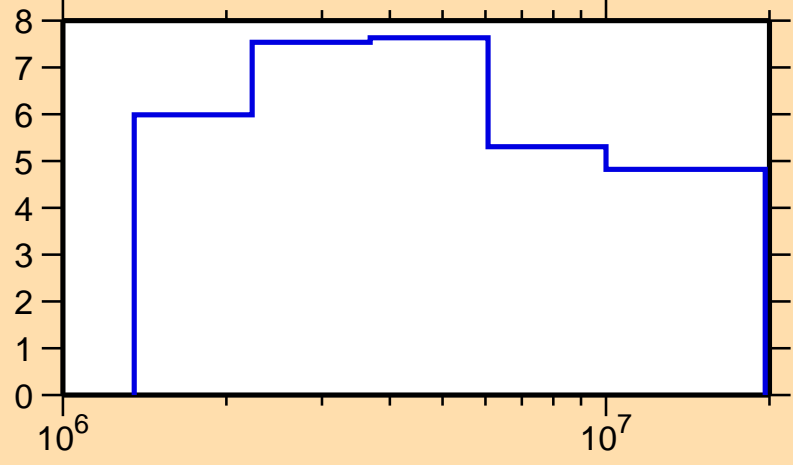
\Delta\sigma/\sigma vs. E for ^{100}\text{Ag}(n,n\text{nonel.})
