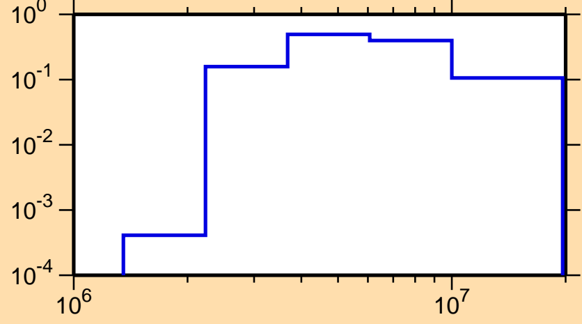
\sigma vs. E for ^{100}\text{Ag}(n,n\text{cont.})
