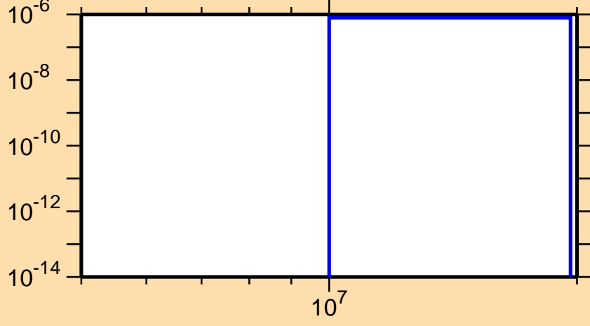
\sigma vs. E for ^{100}\text{Ag}(\text{mt117})
