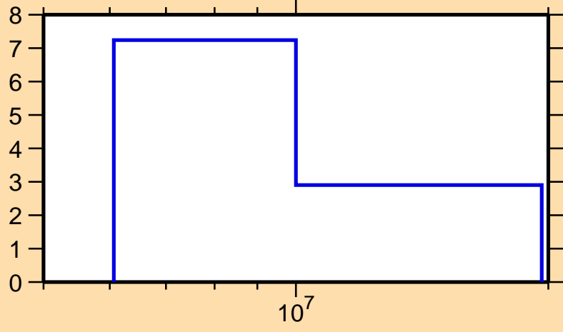
\Delta\sigma/\sigma vs. E for ^{100}\text{Ag}(n,\text{el.})
