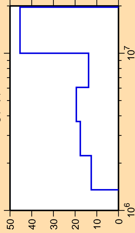
\Delta\sigma/\sigma vs. E for ^{100}\text{Ag}(n,p)
