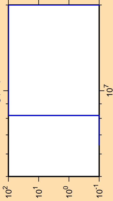
\Delta\sigma/\sigma vs. E for ^{101}\text{Ag}(n,t)
