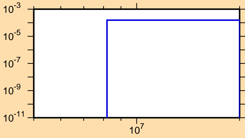
\sigma vs. E for ^{101}\text{Ag}(n,t)
