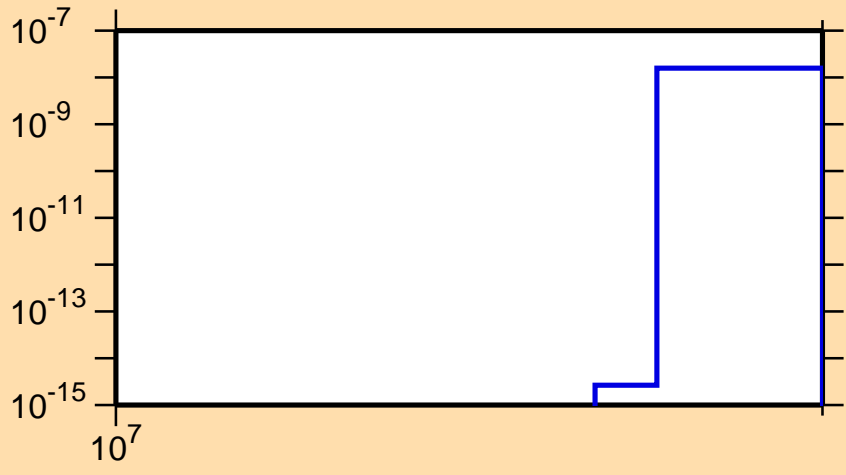
\sigma vs. E for ^{102}\text{Ag}(n,nt)
