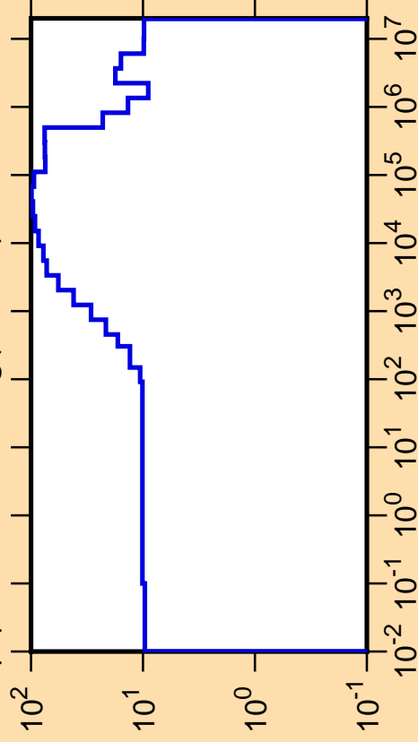
\Delta\mu/\mu vs. E for ^{102}\text{Ag}(\text{mt251})
