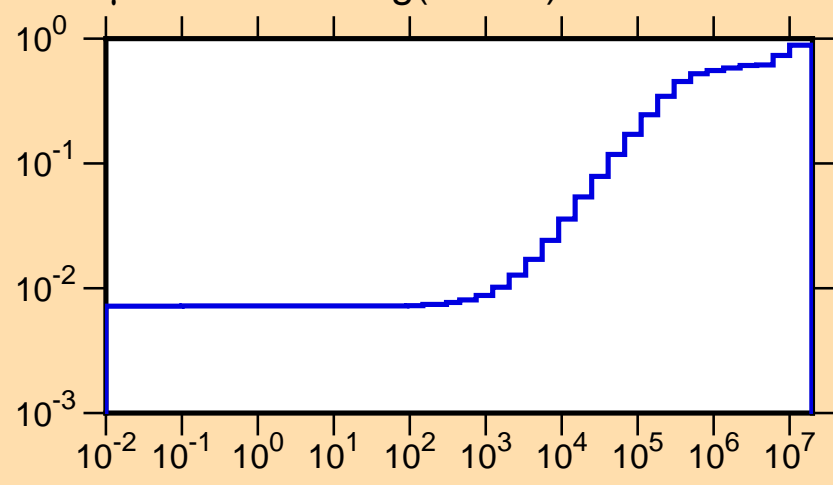
\mu vs. E for ^{102}\text{Ag}(\text{mt251})
