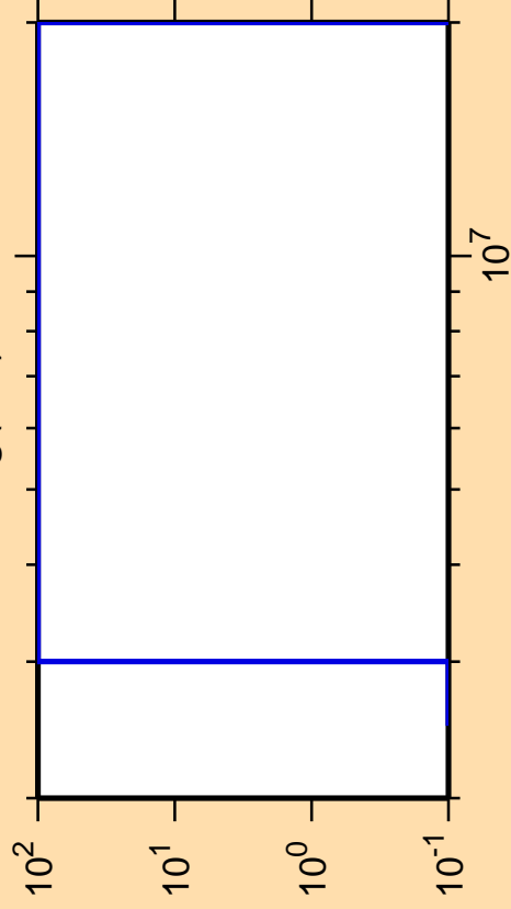
\Delta\sigma/\sigma vs. E for ^{102}\text{Ag}(n,d)
