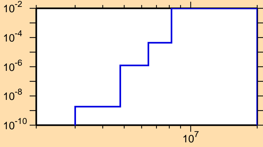
\sigma vs. E for ^{102}\text{Ag}(n,d)
